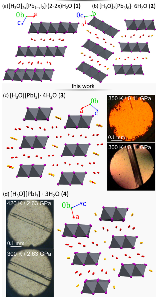
Fig. 1 Four forms of hydrated iodoplumbic acid obtained by reaction of PbI 2 and concentrated aqueous HI: (a) [\text{H}_3\text{O}]_{2x}[\text{Pb}_{1-x}\text{I}_2] \cdot (2-2x)\text{H}_2\text{O} (1, x \approx 0.23 ); (b) (\text{H}_3\text{O})_2\text{Pb}_3\text{I}_8 \cdot 6\text{H}_2\text{O} (2); 30 as well as new materials herein synthesized under high-pressure ( p ) and -temperature ( T ) conditions: (c) (\text{H}_3\text{O})\text{PbI}_3 \cdot 4\text{H}_2\text{O} (3) and (d) (\text{H}_3\text{O})\text{PbI}_3 \cdot 3\text{H}_2\text{O} (4). The proposed sites of H 3 O + cations are marked in orange. Photographs show crystals 3 and 4 in situ grown under pressure.
