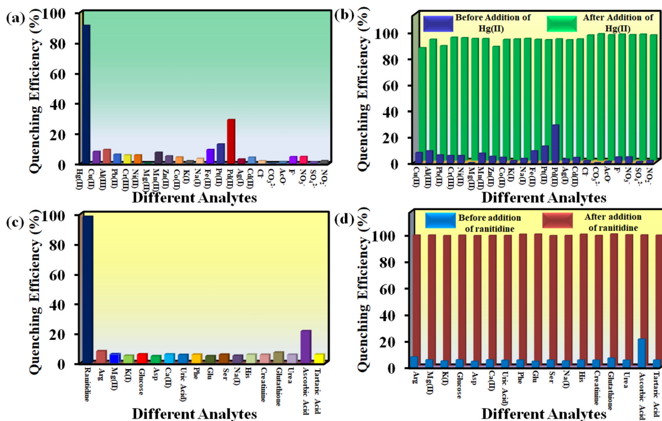
Fig. 4 Selectivity of \mathbf{1}' towards (a) \text{Hg}^{2+} and (c) ranitidine over other analytes and selectivity of \mathbf{1}' towards (b) \text{Hg}^{2+} and (d) ranitidine in presence of other analytes.
