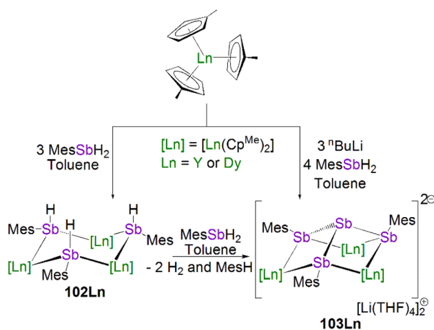
Scheme 33 Synthesis of lanthanide polyantimony complexes 102Ln and 103Ln .
