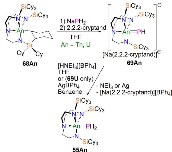
Scheme 22 Synthesis of thorium and uranium phosphinidene complexes 69An and phosphanide complexes 55An .
