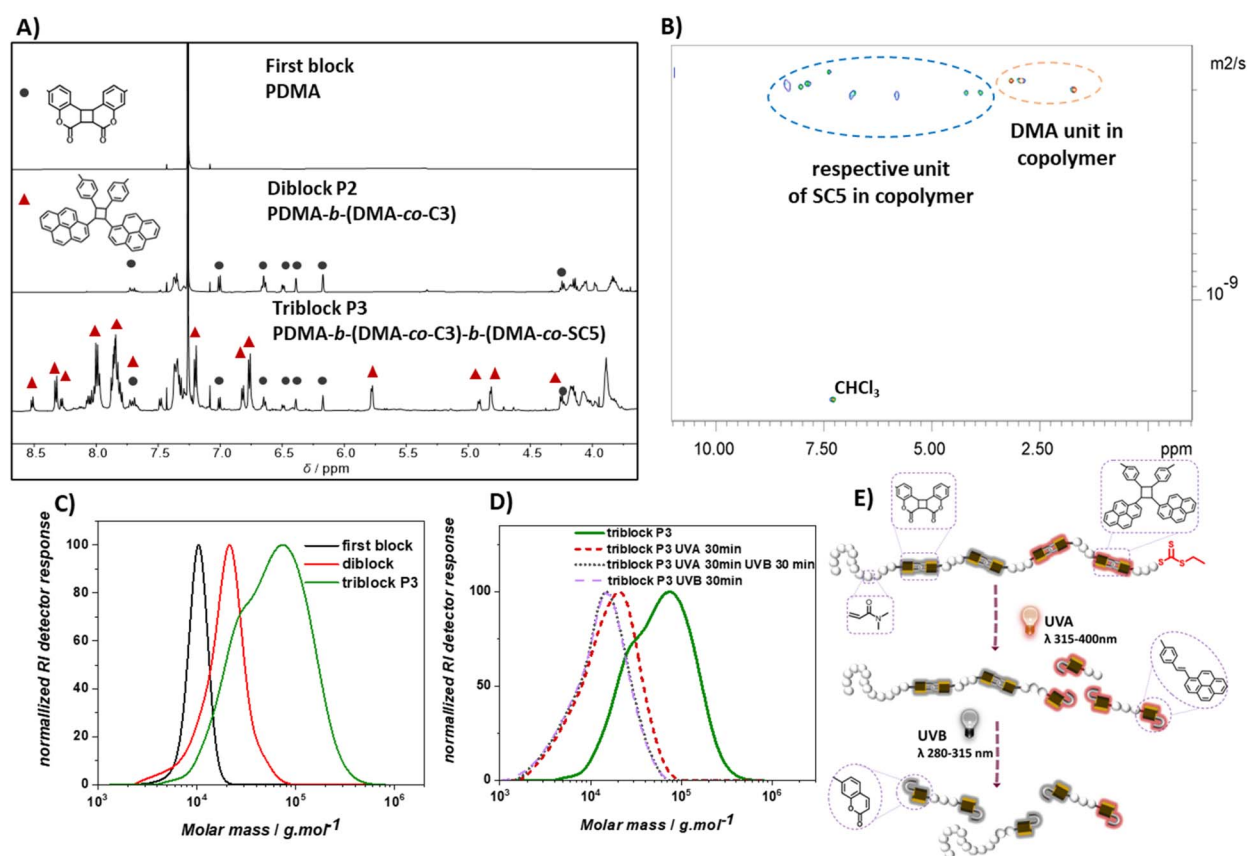
Fig. 4 (A) Stacked 1 H NMR spectra of the homopolymer PDMA, diblock copolymer PDMA- b -(DMA- co -C3) and triblock copolymer P3 PDMA- b -(DMA- co -C3)- b -(DMA- co -SC5); (B) DOSY NMR of polymer P3 showing similar diffusion coefficients for SC5 and DMA resonances, indicative of successful chain extension and copolymerization; (C) overlaid SEC traces of the first block PDMA, diblock polymer and triblock polymer P3; (D) overlaid SEC traces of triblock polymer P3, UVA degraded P3, and UVA-UVB degraded P3; (E) schematic illustration for stepwise UV-degradation of P3 corresponding to photolabile functional groups in each block of the polymer.
