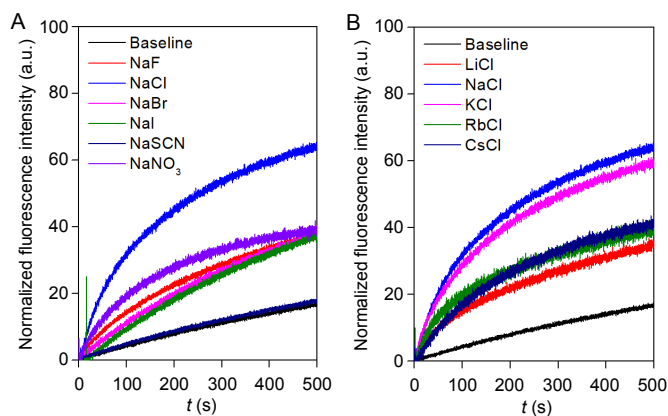
Fig. 4 Ion selectivity of compound 2 across EYPC-LUVs \Rightarrow HPTS towards anion (A); and cation (B) at 300 \text{ nM} concentration.
