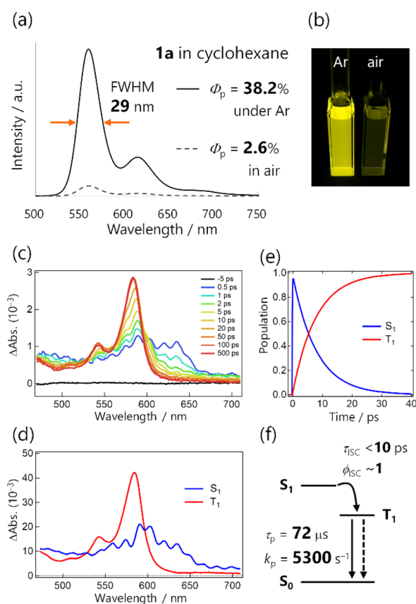
Fig. 2 (a) Steady-state photoluminescence spectra of 1a in cyclohexane ( 4.4 \times 10^{-6} M, excited at 368 nm). (b) Photograph of solutions under 365 nm excitation. (c) fs transient absorption spectra of 1a in cyclohexane excited at 355 nm. (d and e) Selected results from the global analysis based on a sequential model; (d) evolution-associated spectra and (e) corresponding concentration kinetics. Coherent artefact signals are omitted for clarity. (f) Schematic summary of the excited-state dynamics in 1a .
