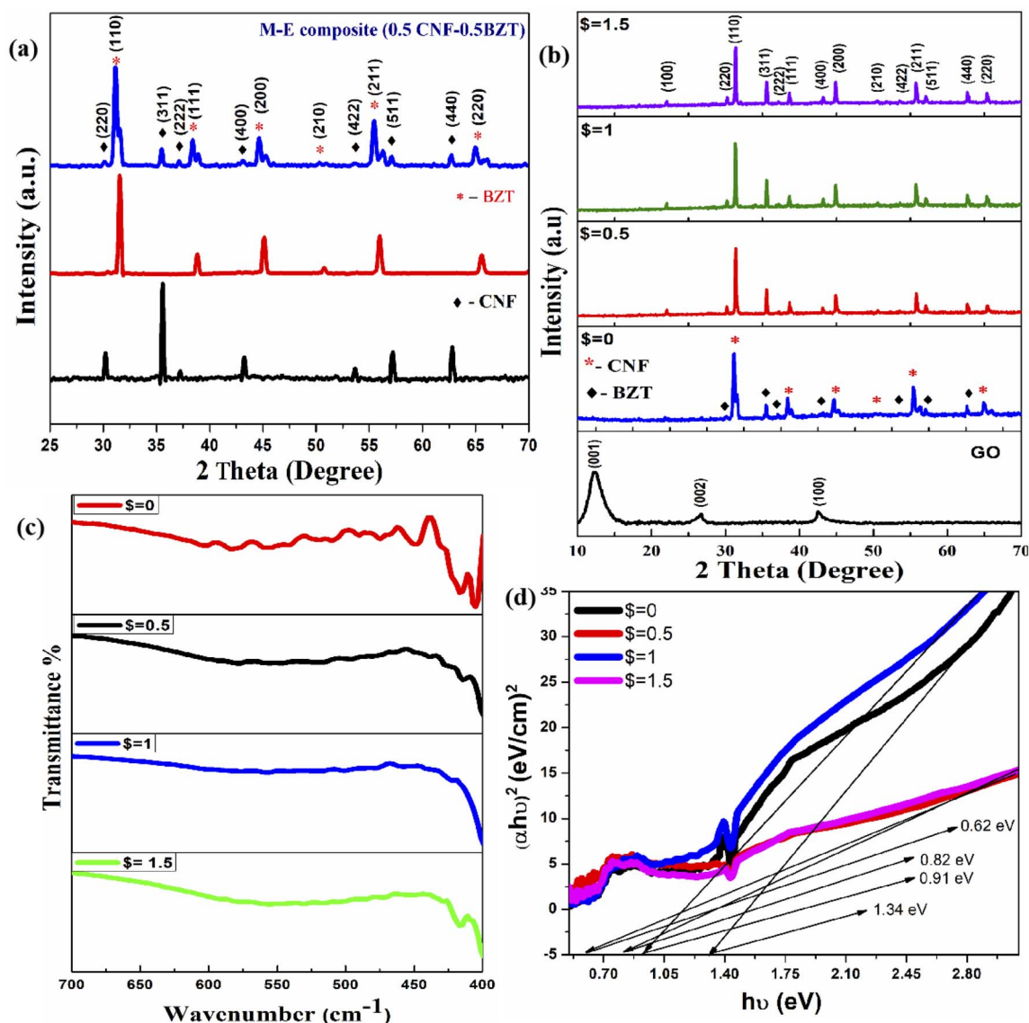
Fig. 2 (a) and (b) XRD pattern for BZT (red line), CNF (black line) and 0.5BZT-0.5CNF-ξ% GO (ξ = 0, 0.5, 1, 1.5) composites. (c) FTIR spectra of GO reinforced 0.5CNF-0.5BZT composites. (d) Tauc's plot to evaluate the band gap energy of 0.5BZT-0.5CNF-ξ% GO (ξ = 0, 0.5, 1, 1.5).
