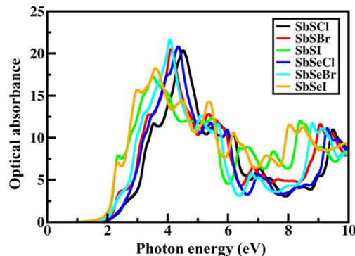
Fig. 7 Optical absorbance of 2D Janus SbYZ ( Y = \text{S, Se} and Z = \text{Cl, Br \& I} ) monolayers using GW-BSE theory.
