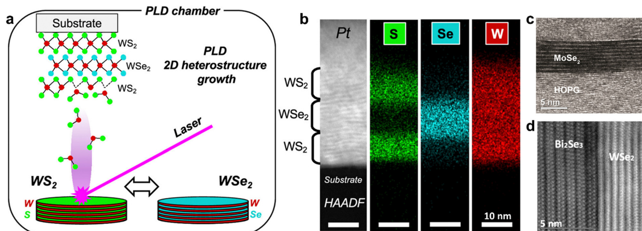
Fig. 3 (a) Schematic of PLD-based VdWE of WS_2/WSe_2 heterostructures; (b) scanning transmission electron microscopy image of 2D WS_2/WSe_2/WS_2 heterostructures fabricated by PLD-based VdWE, with corresponding elemental mapping by electron-dispersive X-ray spectroscopy; (c) transmission electron microscopy image of 9 monolayer MoSe_2 on highly oriented pyrolytic graphite (HOPG) fabricated by MBE. (d) Transmission electron microscopy image of multilayered WSe_2 on single crystal Bi_2Se_3 fabricated by MBE. Panels (a) and (b) are adapted with permission from The American Chemical Society (CC-BY-NC-ND 4.0). 91 Panels (c) 92 and (d) 93 are adapted with permission from IOP Publishing.
