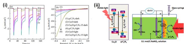
Fig. 8 (i) (a) Transient photocurrent response at a bias potential of -0.4 \text{ V} (vs. \text{Ag}/\text{AgCl} ) under visible light: [(1) \text{Cu}_2\text{O} ; (2) \text{Cu}_2\text{O}/\text{g-C}_3\text{N}_4-5 ; (3) \text{Cu}_2\text{O}/\text{g-C}_3\text{N}_4-10 ; (4) \text{Cu}_2\text{O}/\text{g-C}_3\text{N}_4-15 ; (5) \text{Cu}_2\text{O}/\text{g-C}_3\text{N}_4-20 ; (6) \text{g-C}_3\text{N}_4 ]. (b) Linear sweep voltammograms of \text{Cu}_2\text{O} , \text{g-C}_3\text{N}_4 and \text{Cu}_2\text{O}/\text{g-C}_3\text{N}_4-15 films in the dark and under visible light. (ii) Schematic pathway for photoelectron transfer and the photoelectrochemical process in \text{Cu}_2\text{O}/\text{g-C}_3\text{N}_4 film under visible light irradiation. Reprinted from ref. 151 with permission.
