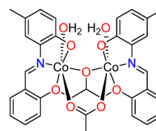
Fig. 1 Structure of the dinuclear Schiff base ORR catalyst [Co 2 (MeBSIP)(OAc)(H 2 O) 2 ] ( 2 ).
