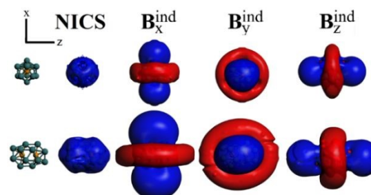
Fig.7. Magnetic response properties of [\text{Pd}_2@\text{Sn}_{18}]^{4-} , denoting the NICS isosurfaces, and from specific orientations of the external field ( B_z^{\text{ind}} , B_y^{\text{ind}} , and B_x^{\text{ind}} ). Isosurfaces set to \pm 3 ppm, blue - shielding; red - deshielding. Reprinted with permission from Ref. 209 . Copyright Royal Society of Chemistry, 2024.
