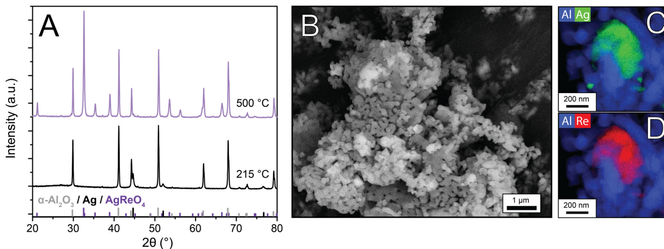
Fig. 4 X-ray diffractograms of the \text{AgReO}_4 samples calcined at 215 and 500^\circ\text{C} , with theoretical stick diffraction patterns of \alpha - \text{Al}_2\text{O}_3 , Ag and \text{AgReO}_4 below (A), SEM image of \text{AgReO}_4/\alpha - \text{Al}_2\text{O}_3 calcined at 500^\circ\text{C} (B) and STEM-EDX maps of a zoomed in \text{AgReO}_4/\alpha - \text{Al}_2\text{O}_3 particle (C and D).
