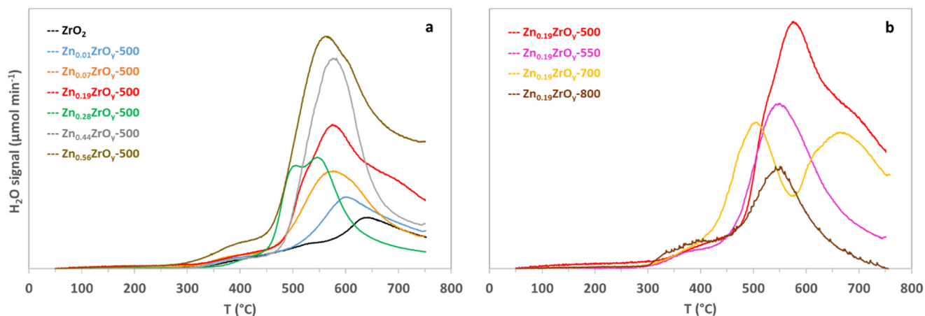
Fig. 4 Temperature-programmed H 2 reduction of (a) Zn x ZrO y -500 catalysts and (b) Zn 0.19 ZrO y -T calcined at 500, 550, 700, and 800 °C.
