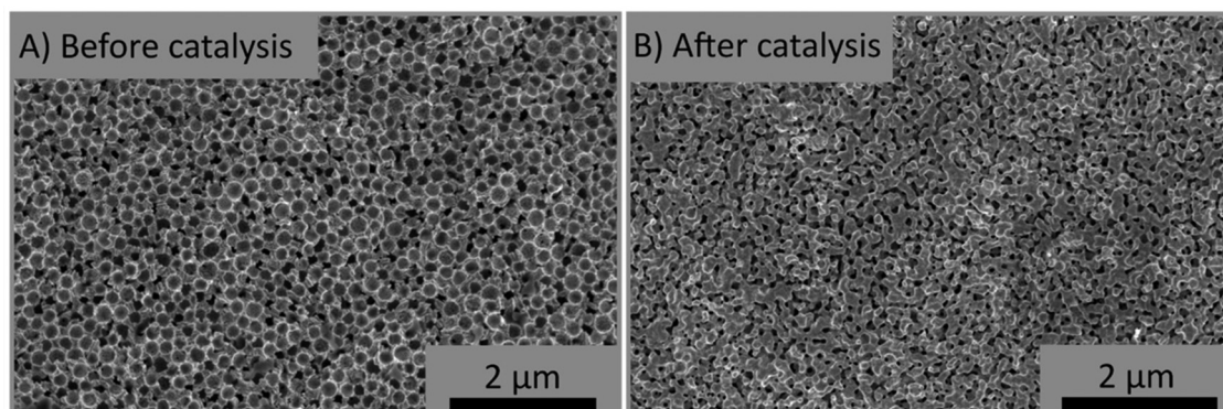
Fig. 9 HR-SEM images of p-flat-default (A) before catalysis and (B) after 1 cycle of catalysis at potentials between -0.65\text{ V vs. RHE} and -1.05\text{ V vs. RHE} .
