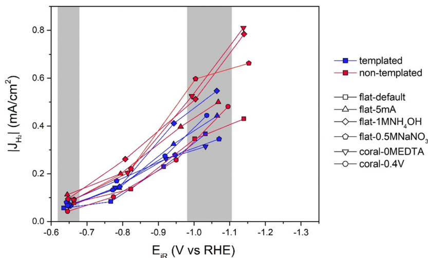
Fig. 7 Partial current densities to \text{H}_2 for both the template-based porous (blue) and non-templated equivalent (red) samples (n)t-flat-default, (n)t-flat-5mA, (n)t-flat-1MNH 4 OH, (n)t-flat-0.5MNaNO 3 , (n)t-coral-0MEDTA and (n)t-coral-0.4V. The areas in gray indicate the datapoints included in Fig. 8(a) and (b).
