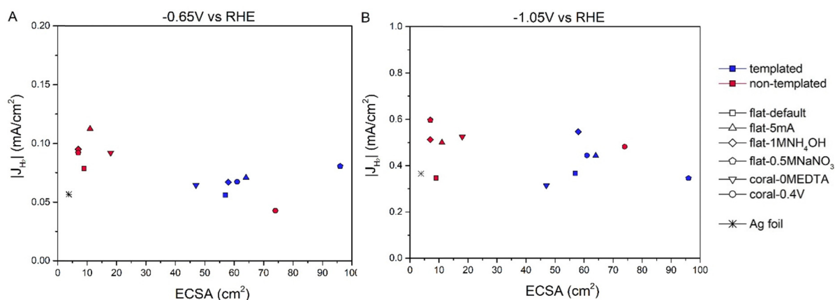
Fig. 8 Partial current densities to \text{H}_2 for both the template-based porous (blue) and non-templated equivalent (red) samples (n)t-flat-default, (n)t-flat-5mA, (n)t-flat-1MNH 4 OH, (n)t-flat-0.5MNaNO 3 , (n)t-coral-0MEDTA and (n)t-coral-0.4V at (A) -0.65\text{ V vs. RHE} and (B) -1.05\text{ V vs. RHE} plotted versus the ECSA.
