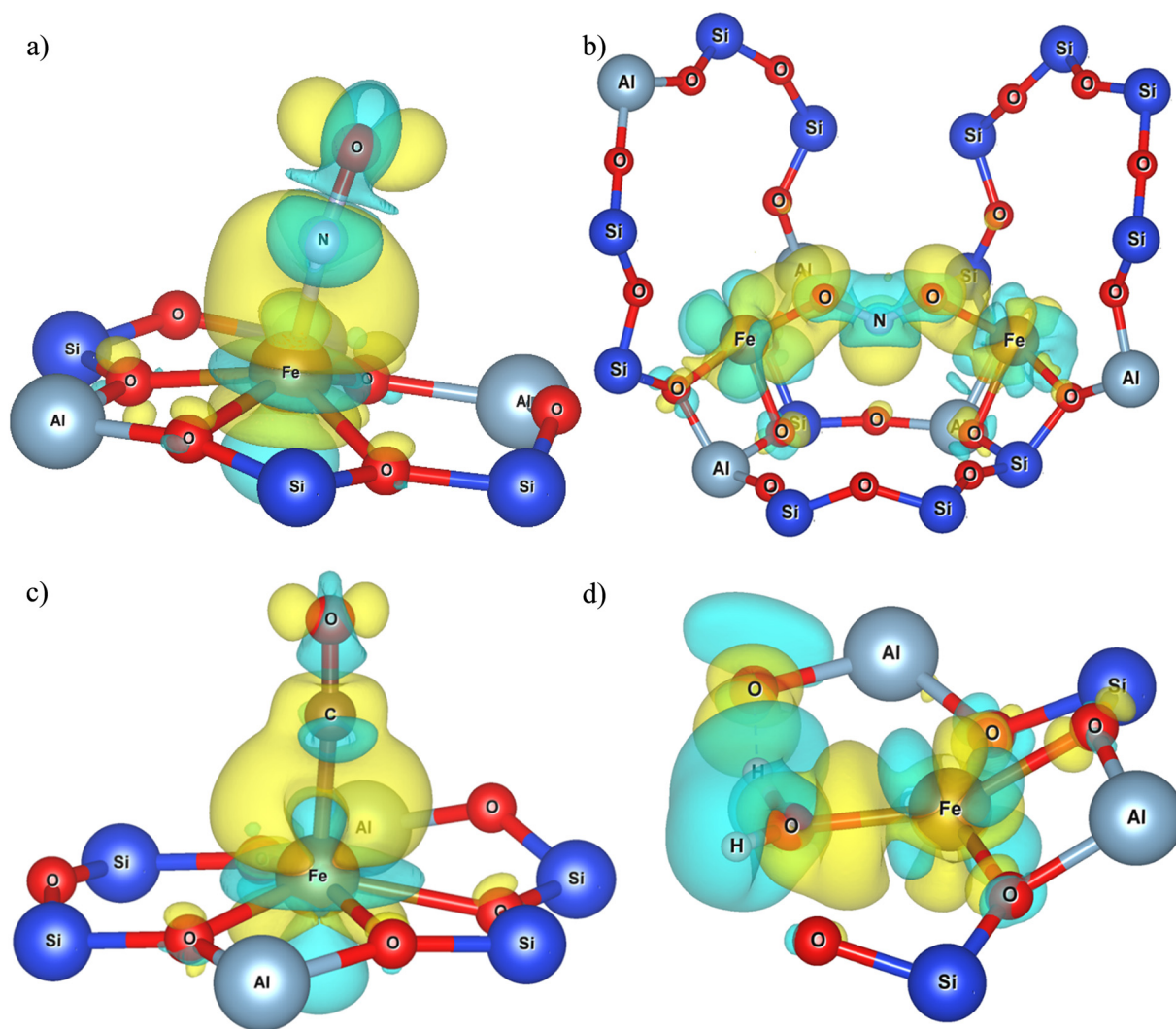
Fig. 8 The charge density differences that occurred during the adsorption on FeCHA-3, of a) NO, b) \text{NO}_2 , c) CO, and d) \text{H}_2\text{O} . The isosurfaces have a density of 0.002 \text{ e/Å}^3 .
