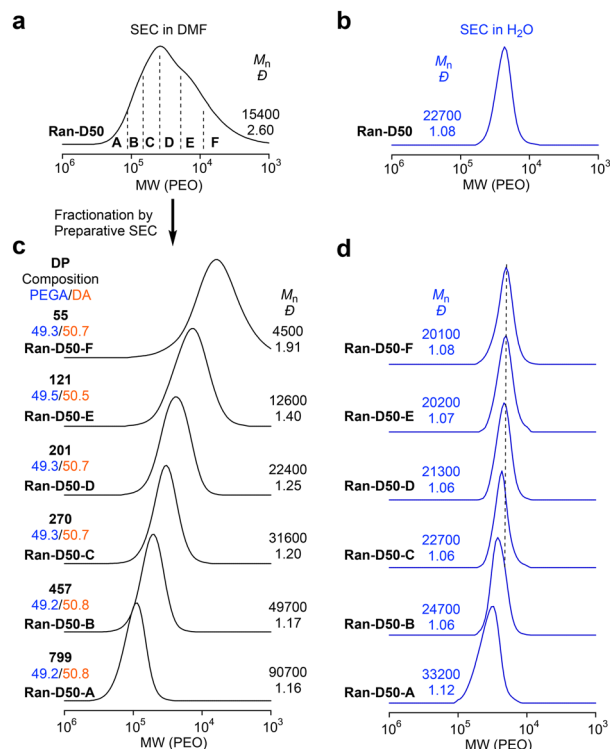
Fig. 2 SEC curves of Ran-D50 in (a) DMF (10 mM LiBr) and (b) H 2 O (100 mM NaCl) with PEO standard calibration. Ran-D50 was fractionated into six samples with different molecular weights ( A–F ) by preparative SEC. (c and d) SEC curves of fractionated Ran-D50-A–F with different DPs in (c) DMF (10 mM LiBr) and (d) H 2 O (100 mM NaCl). The M_n and D values are determined with PEO standard calibration.
