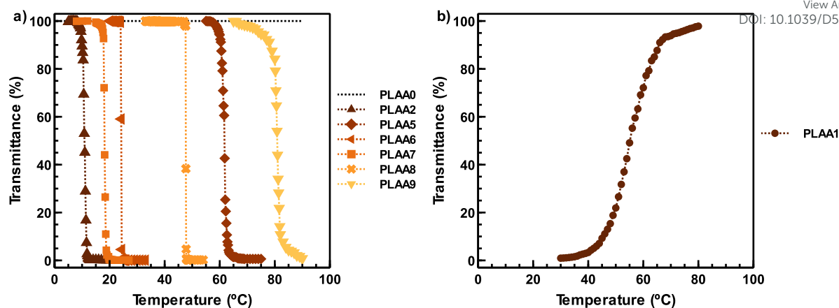
Fig. 2 Temperature-dependent transmittance of (a) LCST-type and (b) UCST-type PLAAAs ( c = 5 \text{ mg}\cdot\text{mL}^{-1} ). See Table 2 for polymerization results.
