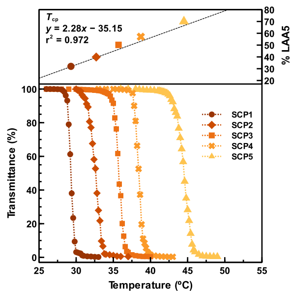
Fig. 3 Temperature-dependent transmittance of SCPs ( c = 5 \text{ mg}\cdot\text{mL}^{-1} ) and relationship between T_{cp} values and LAA5 comonomer content. See Table S1† for statistical copolymerization conditions and results.
