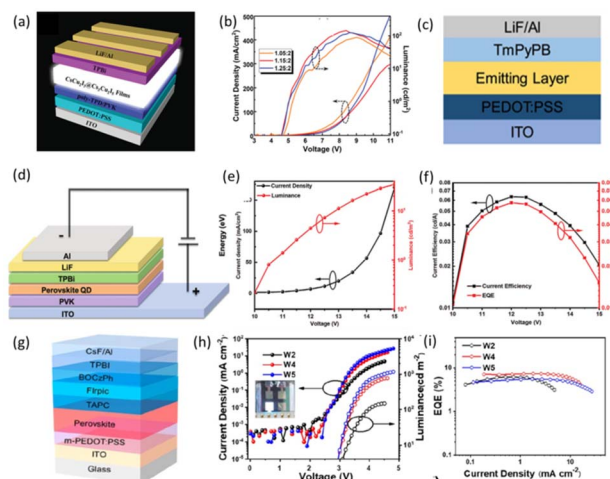
Fig. 8 (a) Schematic structure of the electrically driven WLEDs based on \text{CsCu}_2\text{I}_3@/\text{Cs}_3\text{Cu}_2\text{I}_5 composite films. 104 Copyright 2020 Wiley-VCH. (b) Current density-voltage-luminance curves of WLEDs with different CsI/CuI molar ratios. 104 Copyright 2020 Wiley-VCH. (c) Schematic diagram of the WLED structure. 110 Copyright 2021 Springer Nature. (d) Structure diagram of \text{Cs}_2\text{AgIn}_{0.9}\text{Bi}_{0.1}\text{Cl}_6 QDs-based electroluminescence WLEDs. 111 (e) Dependence of the current density and luminance on the driving voltage. 111 (f) Dependence of the current efficiency and EQE on the driving voltage. 111 Copyright 2021 Wiley-VCH. (g) Schematic diagram of the device structure of the perovskite/organic hybrid white LEDs. 112 (h) J-V-L (inset: photograph of working device W4) and (i) EQE- J characteristics of devices W2, W4, and W5. 112 Copyright 2022 American Chemical Society.
