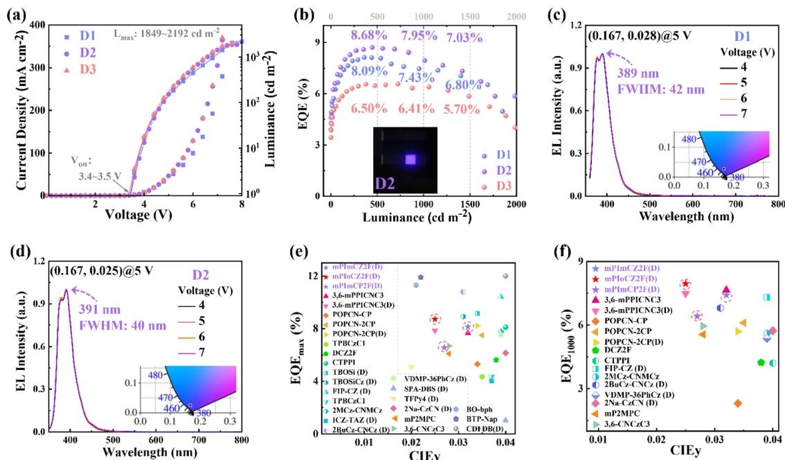
Fig. 6 (a) Current density–voltage–luminance characteristics of the devices D1, D2, and D3. (b) EQE versus luminance curves of the devices D1, D2, and D3 (Inset Photograph of the device D2). (c and d) EL spectra of the devices D1 and D2 at different voltages (Inset CIE coordinates at 5 V). (e and f) Summary of \text{EQE}_{\text{max}} and EQE at 1000 \text{ cd m}^{-2} for the representative reported non-doped and doped (D) fluorescent OLEDs with a \text{CIE}_y \leq 0.04 , and the details are listed in Table S8.†
