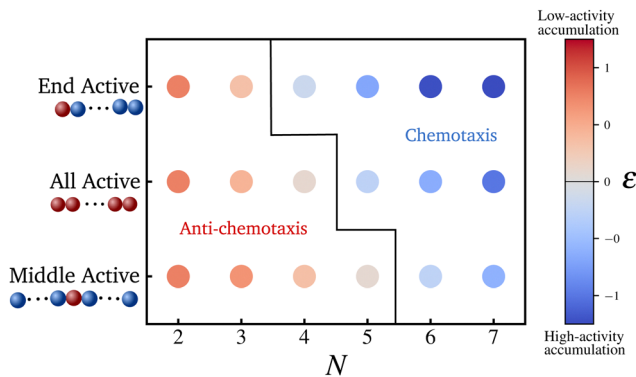
Fig. 3 Scatter plot for \varepsilon which indicates the location and degree of preferential accumulation for three distinct configuration of polymers of various chain length. Values of \varepsilon obtained analytically for the set of parameters mentioned in Fig. 2. As mentioned in the main text, \varepsilon < 0 on the colorbar indicates accumulation in high activity regions, and those greater than zero represent low-activity accumulation.
