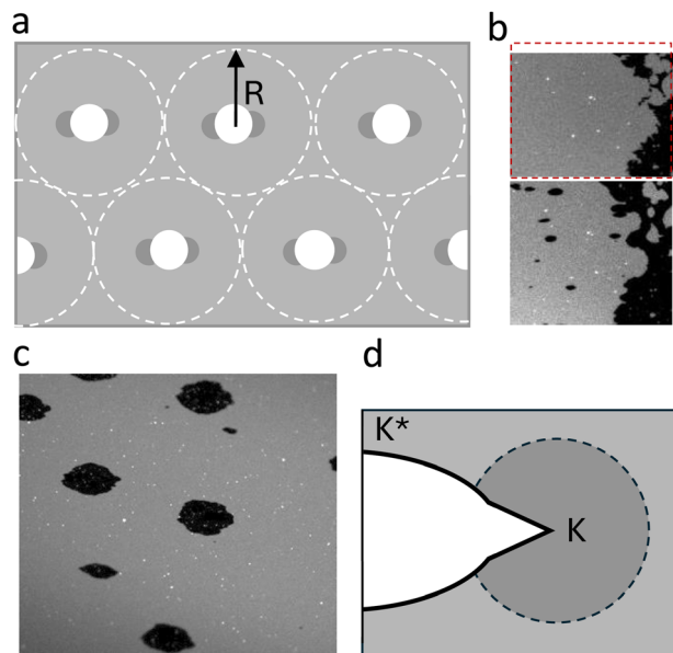
Fig. 4 (a) Schematic drawing of the tension distribution in the membrane, with dark shades of grey indicating stress concentration at the tip of the pores. R corresponds to the tension diffusion length. (b) Microscopic images of a supported lipid bilayer patch made of DOPC lipids before and after the stretch. Full video in ESI.† The red box shows the dimensions of the sample achieved after the stretch. (c) Image of membrane pores with viscoelastic trumpet shapes. Scale bar is 20 \mu\text{m} . (d) Viscoelastic trumpet structure characteristic of the failure behaviour of materials with rate dependent properties. The tip of the crack is characterised by large tension, high elastic modulus ( K ), and a sharp crack propagation. Away from the pore tip, membrane behaves as a deformable material with lower elastic modulus, K^* .
