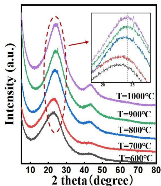
Fig. 1 The XRD patterns of the various samples.
