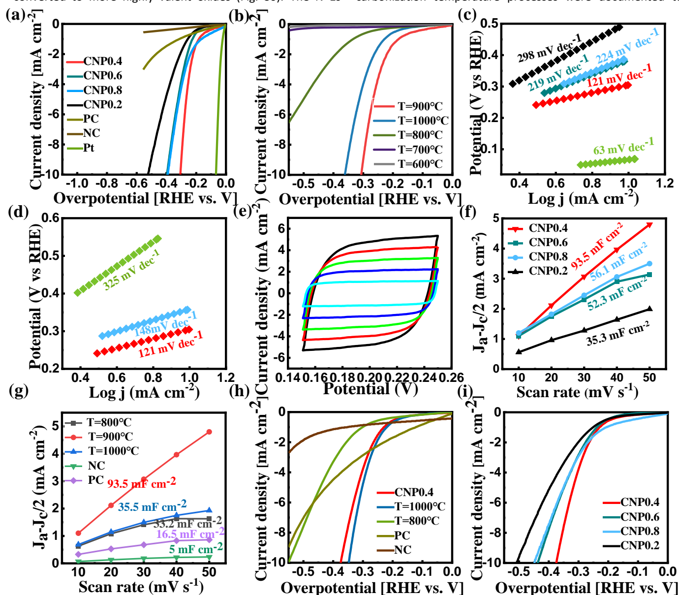
Fig 4. (a,b) The LSV curves of the various samples . (c,d) The corresponding tafel slopes. (e) The CV curves of CNP0.4 in 0.5M H_2SO_4 with the sweep rate changed from 10 mV s^{-1} to 50 mV s^{-1} . (f) The ESCA of sample CNP0.2, CNP0.4, CNP0.6 and CNP0.8. (g) The ESCA of sample T=800 °C, 900 °C, 1000 °C, PC and NC. (h) The normalized current density of sample T=800 °C, 900 °C, 1000 °C, PC and NC. (i) The normalized current density of CNP0.2, CNP0.4, CNP0.6 and CNP0.8.
