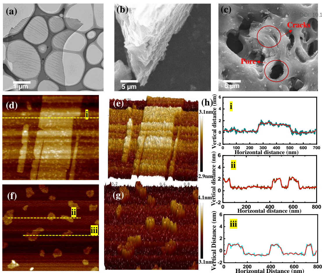
Fig 2. (a) The TEM image of sample CNP0.4. (b) The SEM image of sample CNP0.4 from the side view. (c) The SEM image of sample CNP0.4 from the top view. (d) AFM image of CNP0.4 at micro meter scale and (e) The corresponding 3D height distribution. (f) AFM image of CNP0.4 at nano meter scale and (g) the corresponding 3D height distribution. (h) The height of line i,ii and iii in AFM images.
