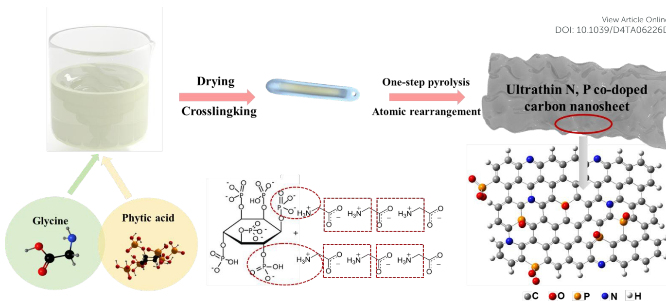
Scheme 1. Schematic representation of synthetic method for CNP.
