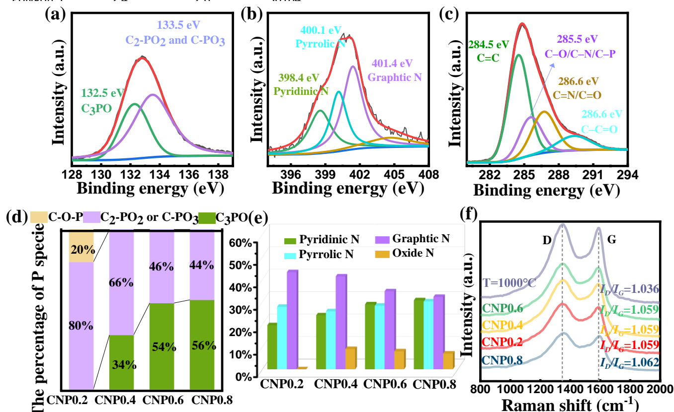
Fig 3. (a) The P 2p spectrum of CNP0.4. (b) the N 1s spectrum of CNP0.4. (c) the C 1s spectrum of CNP0.4. (d) The P species percentage of CNP0.2, CNP0.4, CNP0.6 and CNP0.8. (e) The N species percentage of CNP0.2, CNP0.4, CNP0.6, CNP0.8 and (f) Raman spectra of various samples.
