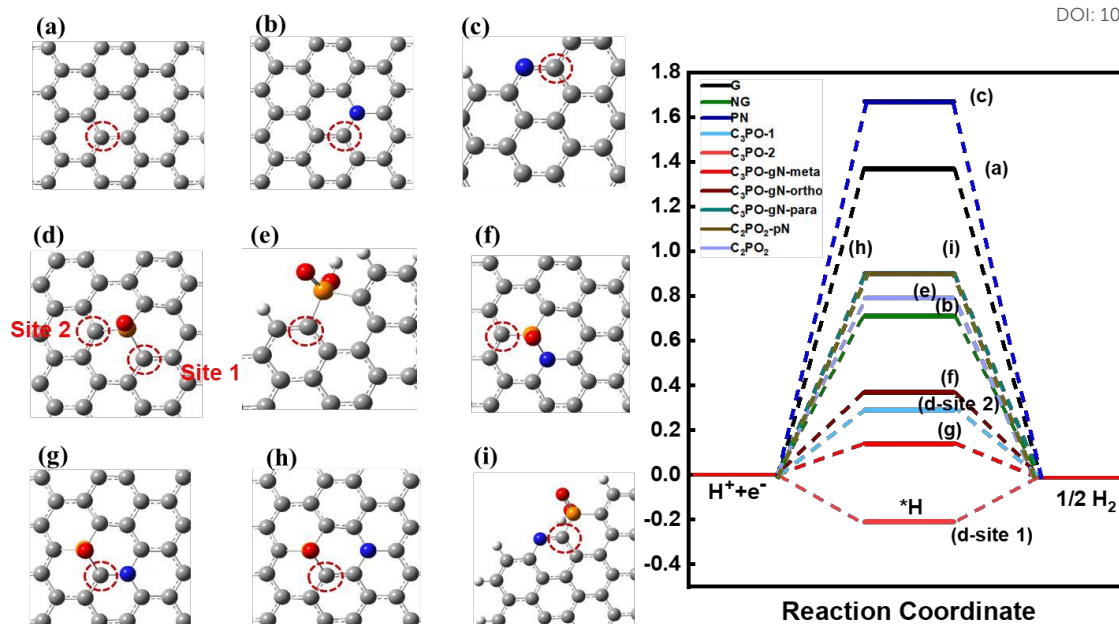
Fig 7. \Delta G_{H^+} of (a) Graphene(G), (b) Graphitic N (NG), (c) Pyridinic N (PN), (d) Graphene doped with C_3PO , (e) Graphene doped with C_2PO_2 (f) Graphene doped with C_3PO and graphitic N in ortho site( C_3PO -gN-ortho). (g) Graphene doped with C_3PO and graphitic N in meta site( C_3PO -gN-meta). (h) Graphene doped with C_3PO and graphitic N in para site( C_3PO -gN-para). (i) Graphene doped with C_2PO_2 and graphitic N ( C_2PO -pN).
