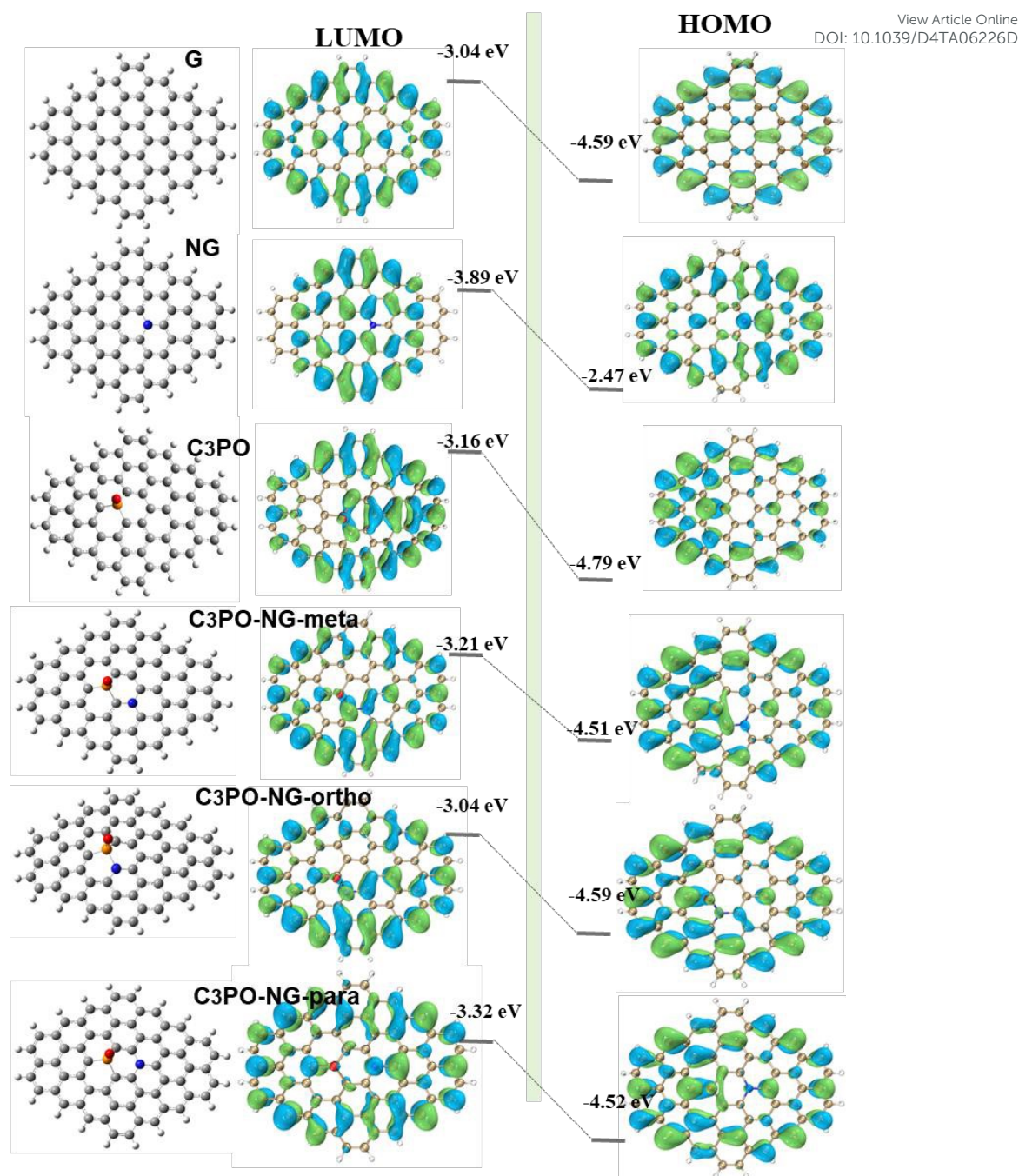
Fig 8. The HOMO and LUMO orbitals of the various models.
