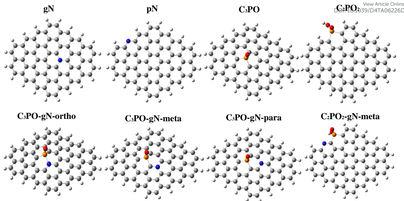
Fig 5. 8 optimized models for the heteroatoms doped graphene.
