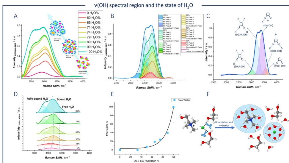
Figure 5 – (A) Spontaneous Raman spectra in the \nu(\text{OH}) region, for DESEG-H 2 O hybrid electrolytes with the indicated water fractions. (B) The fitted Raman spectra of Panel (A). (C) Schematic diagram of water environment and Raman peak assignment. (D) Translated fitted Raman spectra of panel (B) (E) The proportions and total of bulk free H 2 O as a function of the water fraction. (F) Schematic of the coordination environment of DESEG before and after hydration. The white, gray, red, blue, green, balls represent hydrogen, carbon, oxygen, nitrogen atoms and chloride anion, respectively.
