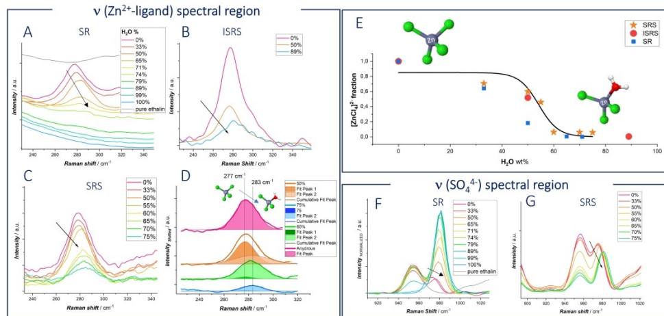
Figure 4 – (A-D) \nu(\text{Zn-Ligand}) and (F-G) \nu(\text{SO}_4^{2-}) spectra for pure anhydrous ethaline and DESEG-H 2 O hybrid electrolytes with the indicated water wt%: (A) spontaneous Raman ; (B) Impulsive Stimulated Raman Scattering (ISRS); (C) Stimulated Raman Scattering (SRS); (D) fitted SRS curves. (E) [\text{ZnCl}_4]^{2-} fraction estimated for the fitting of the spectra of Panels (A-D). (F) Spontaneous Raman. (G) SRS.
