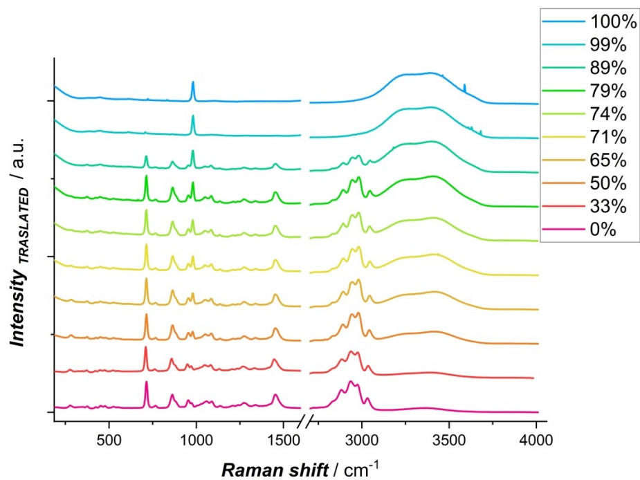
Figure 3 - Spontaneous Raman spectra of DESEG-H 2 O hybrid electrolytes with different wt% (0%, 50%, 65%, 71%, 74%, 79%, 89%, 99% and 100%); the spectra are shifted vertically for clarity.
