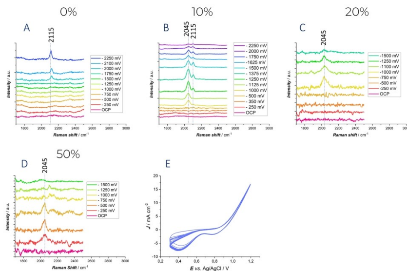
Figure 6 - Potential-dependent in situ SERS spectra measured at an ORC-treated polycrystalline Au electrode in contact with the Ethaline DES with the indicated water contents. Panels (A-D) report the spectra recorded in the CN- stretching range for different hydration levels. (E) A typical ORC cycle adopted for the achievement of the SERS effect.
