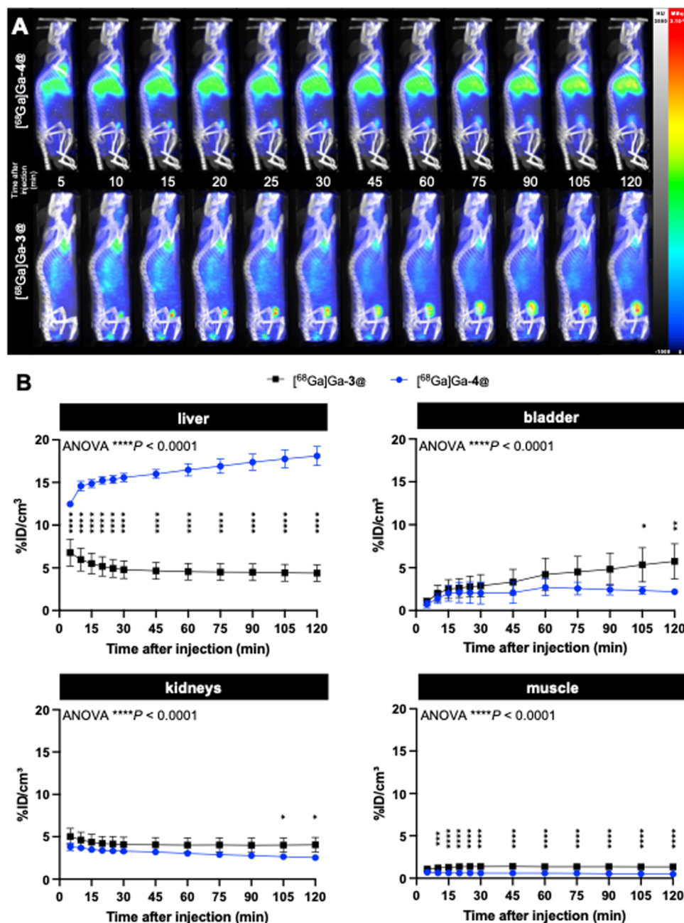
Fig. 5 Dynamic PET/CT biodistribution of [^{68}\text{Ga}]\text{Ga-4@} and [^{68}\text{Ga}]\text{Ga-3@} up to 2 h after intravenous injection in healthy mice ( n = 4 ): (A) representative images and (B) PET quantifications of uptake in the liver, bladder, kidney and muscle over time, analyzed using a 2-way ANOVA followed by Šidák's post-hoc test. * P < 0.05 ; ** P < 0.01 ; *** P < 0.001 ; **** P < 0.0001 .
