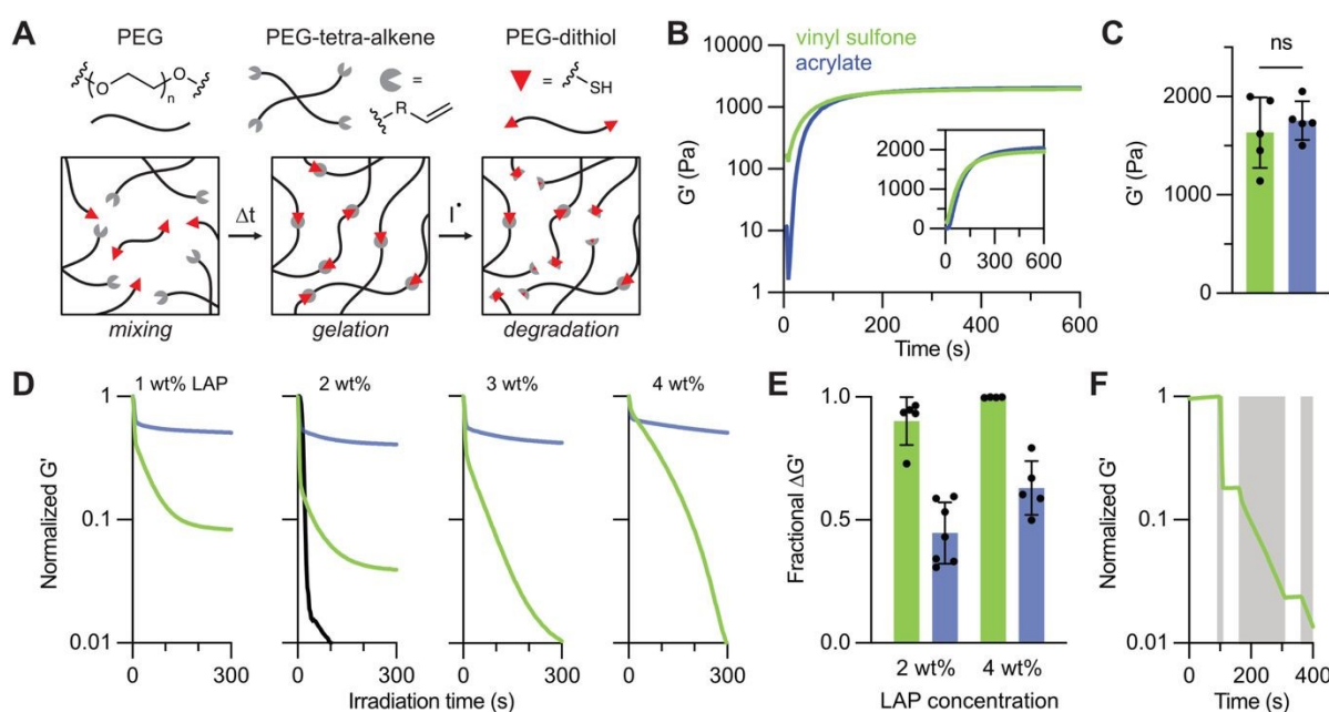
Fig. 3 | Radical-mediated degradation of thiol-Michael hydrogels formed by vinyl sulfones and acrylates. (A) Schematic of network formation via thiol-Michael addition and subsequent degradation by radical species ( I^* ). (B) In situ rheology during gelation shows similar crosslinking kinetics for vinyl sulfone (green) and acrylate (blue) hydrogels with (C) comparable plateau storage moduli. (D) In situ photodegradation profiles at varying LAP concentrations (1-4 wt%) reveal dramatically increased radical susceptibility in vinyl sulfone gels. For the 2 wt% condition, a matched thiol-maleimide gel (black) is included. The change in degradation profile between 3 and 4 wt% LAP for the vinyl sulfone hydrogels may relate to the optical thickness of these samples. (E) A summary of degradation extent at 2 and 4 wt% LAP demonstrates the
