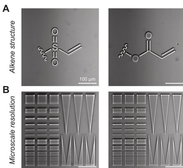
Fig. 4 | Microscale patterning of thiol-Michael hydrogels. (A) Photopatterns of alkene structure formed by rastered laser exposure in vinyl sulfone (left) and acrylate (right) gels containing 4 wt% LAP. (B) Resolution test demonstrating high-fidelity formation of both positive and negative features at the micron scale for both systems (vinyl sulfone left, acrylate right). Quantification shown in Fig. S12.
