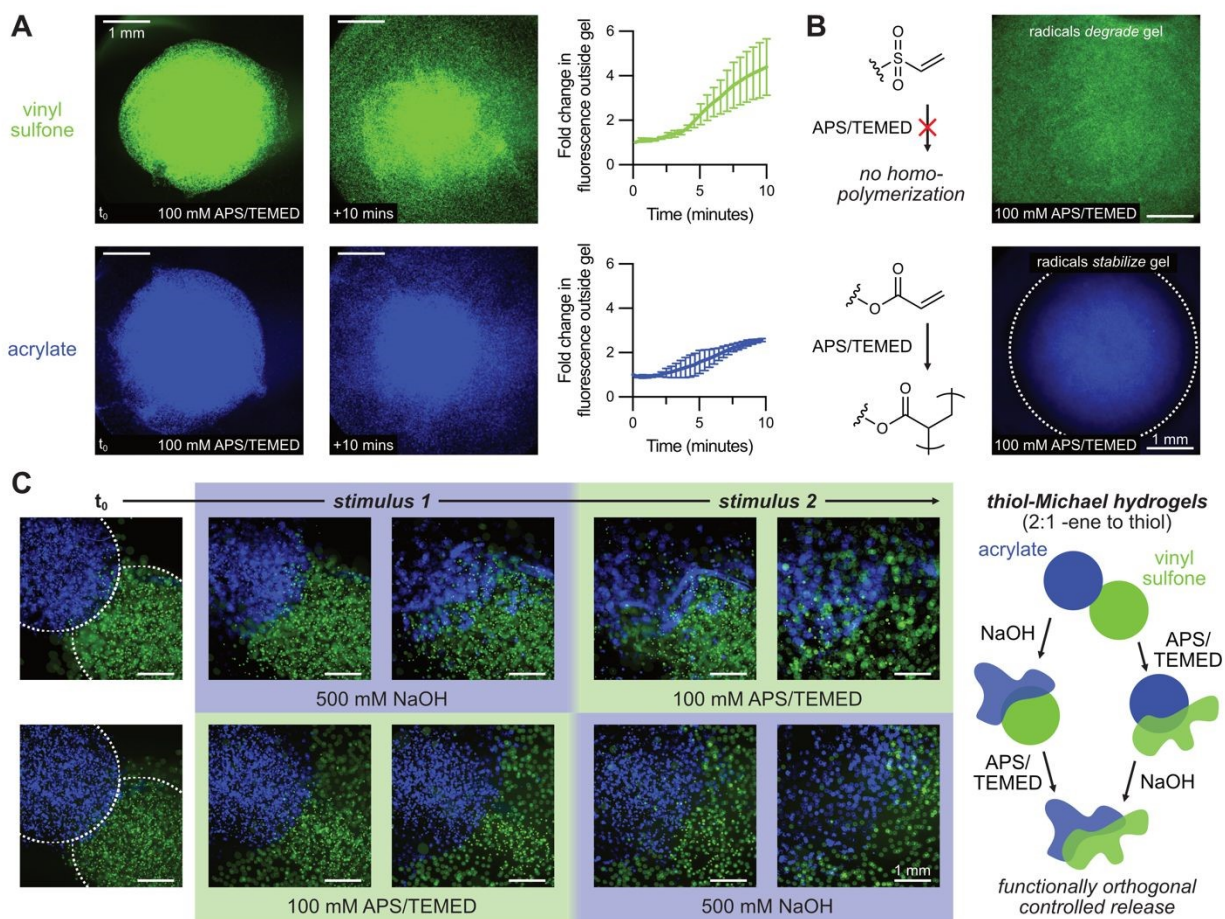
Fig. 5 | Orthogonal degradation of thiol-Michael hydrogels by redox-initiated radicals and hydrolysis. (A) Fluorescent microbeads embedded in thiol-Michael hydrogels are rapidly released upon introduction of redox initiator (APS/TEMED), confirming radical-mediated degradation of both vinyl sulfone (green) and acrylate (blue) gels. (B) In gels formed with excess alkene (2:1 alkene:thiol), redox-initiated radicals selectively degrade vinyl sulfone gels while acrylate gels remain intact 40 minutes after the addition of APS/TEMED, consistent with acrylate homopolymerization-based network stabilization. (C) Sequential treatment with radicals or base revealed functionally orthogonal degradation responses in 2:1 alkene:thiol gels, wherein NaOH selectively degrades acrylate gels while preserving vinyl sulfone networks, and APS/TEMED causes the inverse, enabling pathway-independent and chemically encoded degradation modes.
