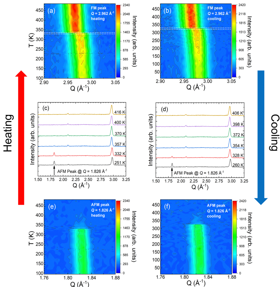
Fig. 2 Contour map of the high-intensity FM/nuclear peak of the neutron diffraction patterns (a) on heating from 100 to 485 K and (b) on cooling from 485 to 10 K. Evolution of the high-intensity AFM peak with temperature, (c) heating and (d) cooling. Contour map of the high-intensity AFM peak of the neutron diffraction patterns (e) on heating from 100 to 485 K, and (f) on cooling from 485 to 10 K. The white horizontal dashed lines in (a) and (b) show the first-order AFM–FM and FM–AFM phase transition ranges, respectively.
