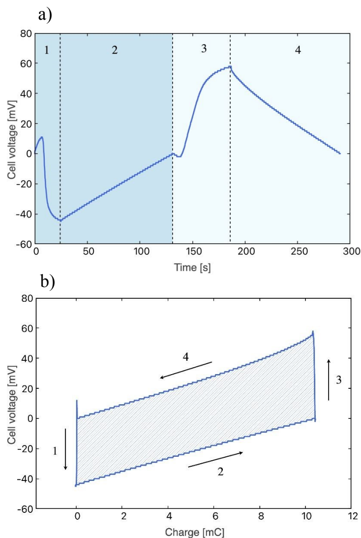
Figure 3. a) Electric potential as a function of time for each CDP stage: 1- Salty water, open circuit; 2- Salty water; closed circuit, applied current value of 0.1 mA; 3- Fresh water, open circuit; 4- Fresh water, closed circuit, applied current value of -0.1 mA. Stages with salty water are marked in dark colour, as the ones with fresh water are coloured in light blue. b) Electric potential evolution with respect to the accumulated charge. The area enclosed by the curves is equal to the energy obtained in the cycle.
