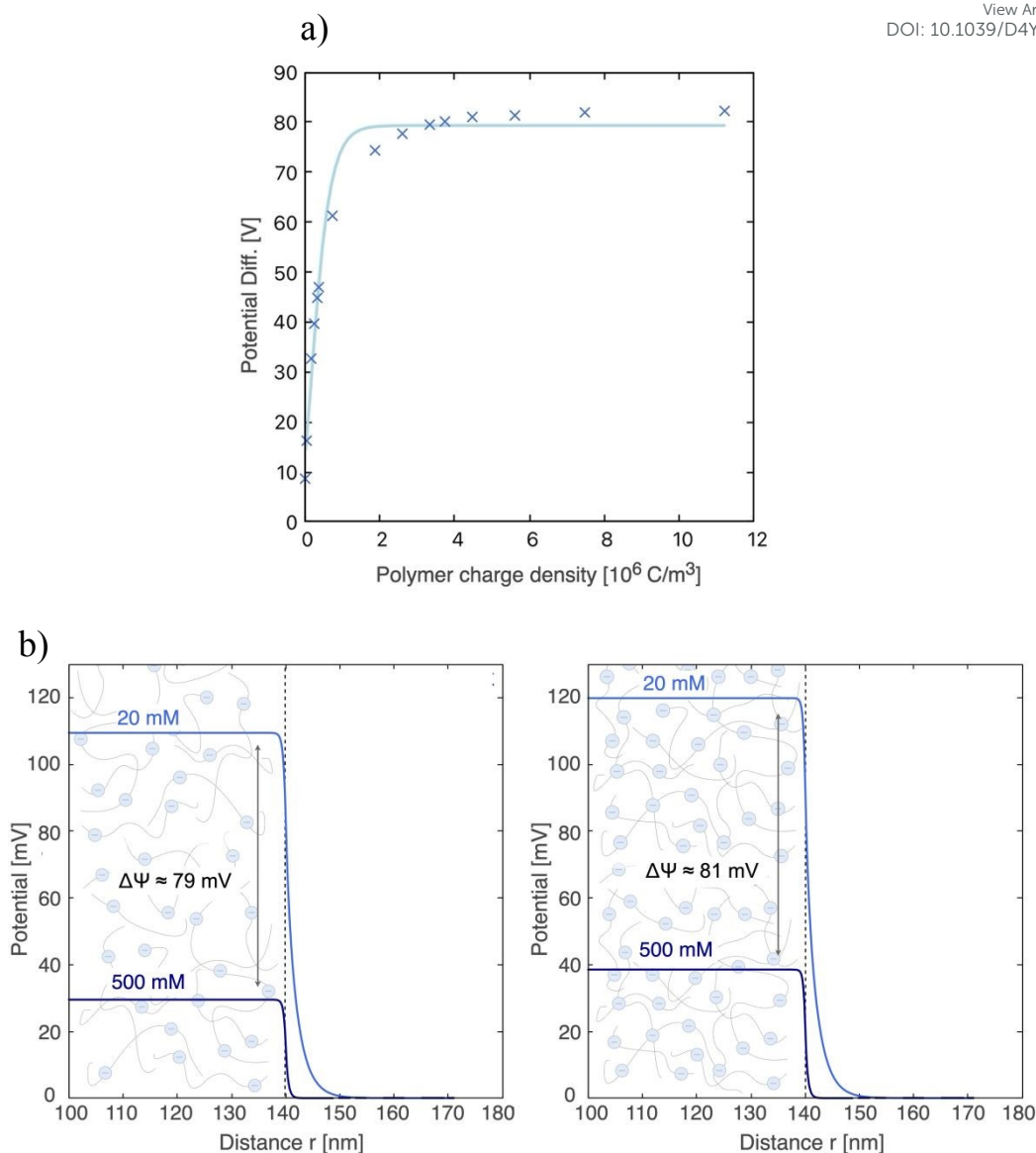
Figure 4. a) Variation of the Donnan potential differences between 20 mM and 500 mM NaCl solutions for two NaCl solutions as a function of the volume charge density of the polymer, \rho_p . b) Electric potential profiles for a spherical particle 100 nm in radius Donnan potential profiles next to the surface of an electrode (thickness of 100 nm) coated with a polymer layer of length L_p = 40 \text{ nm} obtained for 20 mM (light blue) and 500 mM (dark blue) NaCl solutions. The polyelectrolyte charge densities used were \rho_p = 3.7 \times 10^6 \text{ C/m}^3 (left graph) and 5.6 \times 10^6 \text{ C/m}^3 (right graph), giving rise to potential differences of 79 mV and 81 mV, respectively.
