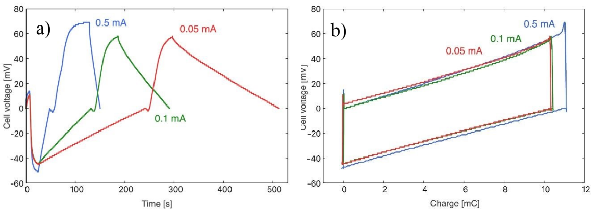
Figure 5. Electric potential difference between electrodes as a function of time (a) and electric potential evolution with respect to the accumulated charge (b) for the different current values used: 0.05 mA (red), 0.1 mA (green) and 0.5 mA (blue).
