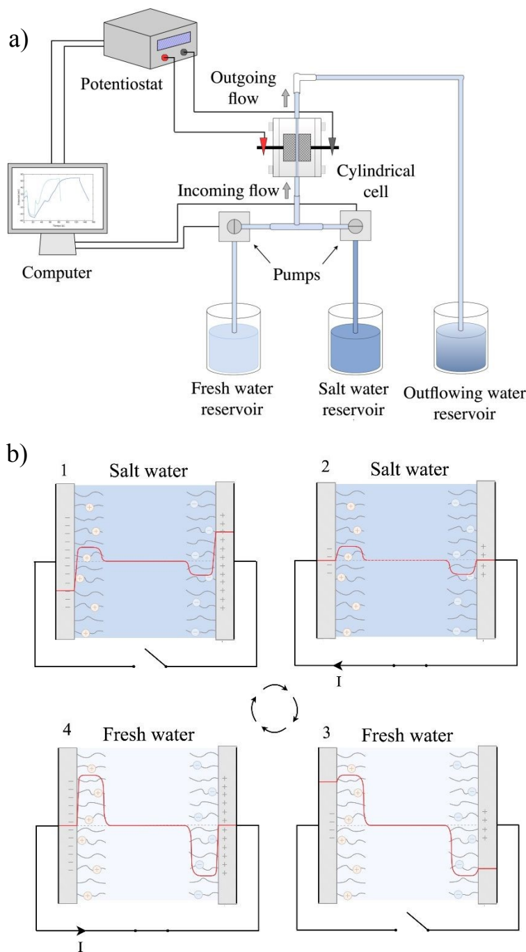
Figure 2. a) Scheme of the experimental setup required for the salinity exchange energy extraction process. b) Potential profile during energy extraction cycle divided in four stages: 1- Salty water, open circuit; 2- Salty water; closed circuit, applied positive
