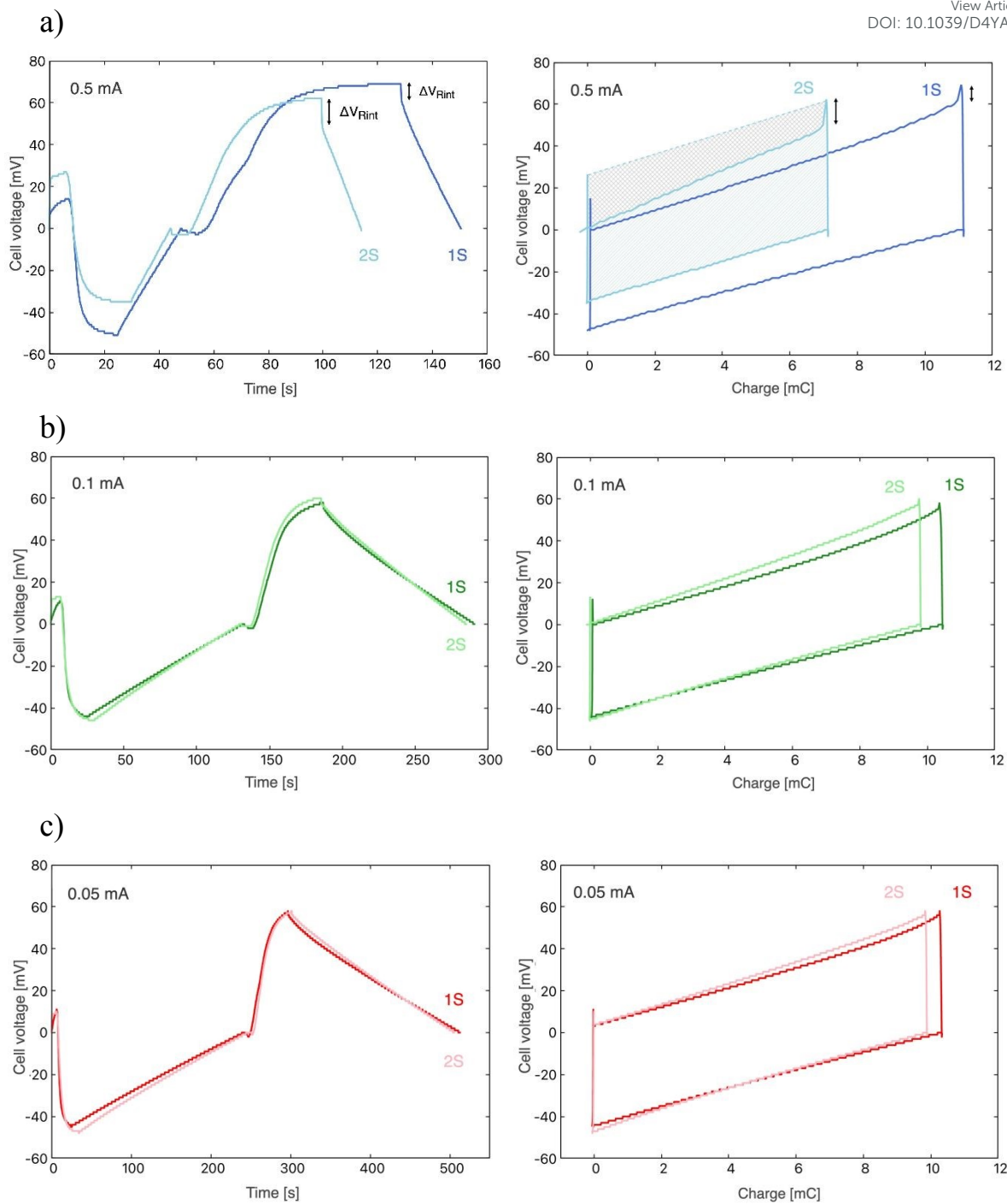
Figure 7. Electric potential as a function of time (left) and electric potential evolution with respect to the accumulated charge (right) for the two electrode separations 1S (dark coloured line) and 2S (light coloured line), and for the different current values used: 0.5 mA (a), 0.1 mA (b) and 0.05 mA (c).
