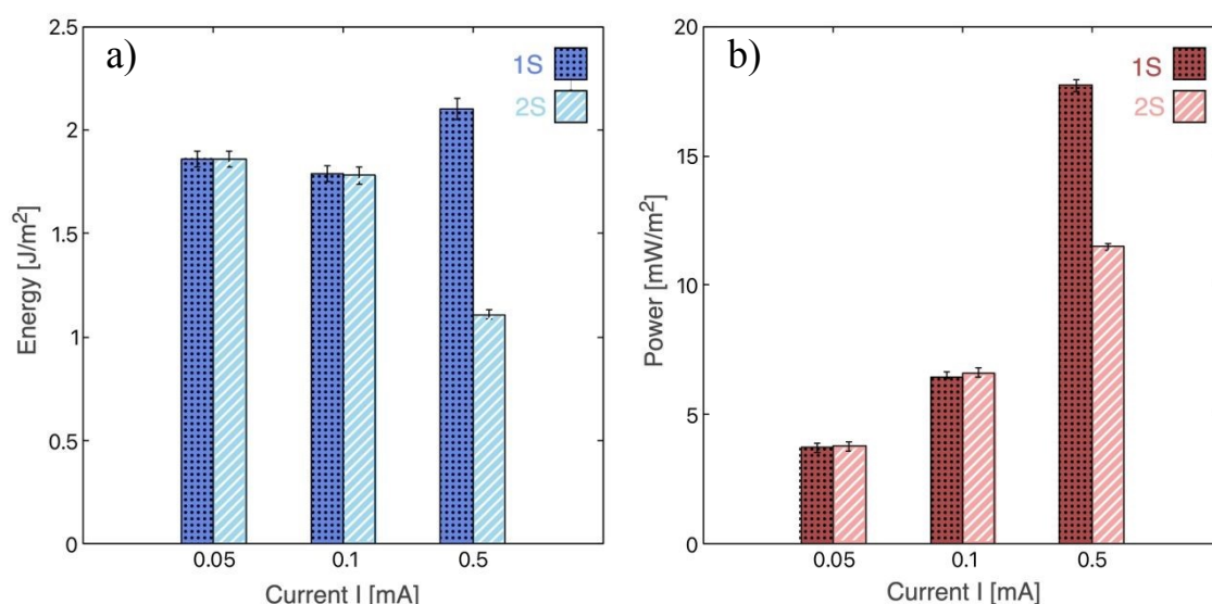
Figure 8. Energy per cycle and per unit area (a) and power generated per unit area (b) as a function of the applied current for each spacer separation used: 1S (darker colour) and 2S (lighter colour).
