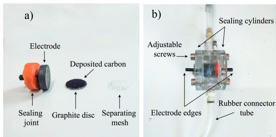
Figure 1. a) Photography of the electrodes and the mesh spacer. b) Measurement cell setup composed of the facing electrodes inside the methacrylate structure and the connector tubes for solution inlet and outlet.
