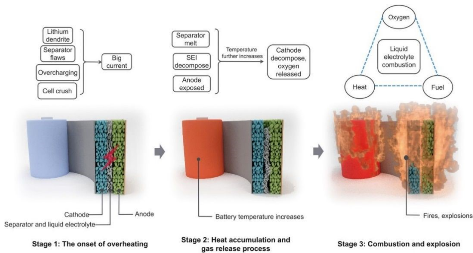
Figure 1: The stages of thermal runaway in LIBs. Reproduced with permission from. 4 Copyright 2018, American Association for the Advancement of Science.
