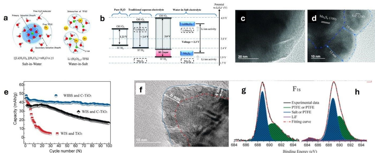
Figure 25: Performance of WiSE Reproduced with permission from. 357 Copyright 2015, American Association for Advancement of Science: a) illustration of the evolution of the Li + primary solvation sheath in diluted vs water-in-salt solutions, b) illustration of expanded electrochemical stability window for water-in-salt electrolytes paired with LiMn 2 O 4 cathode and Mo 6 S 8 anode, b), TEM images of pristine Mo 6 S 8 (c) and cycled Mo 6 S 8 (d) in WiSE electrolyte. Performance of WBS electrolytes. Reproduced with permission from. 358 Copyright 2016, Wiley-VCH: e) Cycling stability of LiMn 2 O 4 ||c-TiO 2 /TiO 2 anodes in 12m LiTFSI in water (WIS) and 21m LiTFSI + 7m LiOTf (WBS) electrolytes, f) TEM images of C-TiO 2 recovered after 143 cycles in WBS at 1 C, g) and h) XPS of C-TiO 2 anode before and after 10 cycles at 0.5 C, respectively in WBS electrolyte.
