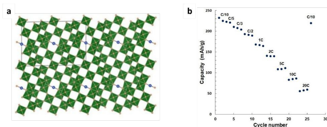
Figure 4: a) Crystal structure of NaNb 13 O 33 viewed down the b-axis. Green octahedra represent Nb-centered NbO 6 . Na atoms are in blue, O atoms in orange. b) Delithiation capacity as a function of the rate of NaNb 13 O 33 with high-rate capability up to 20C in a Li metal half-cell at the indicated charge-discharge rates. Reproduced under the terms of the Creative Commons CC BY license. 118 Copyright 2023, The Authors. ChemElectroChem published by Wiley-VCH GmbH
