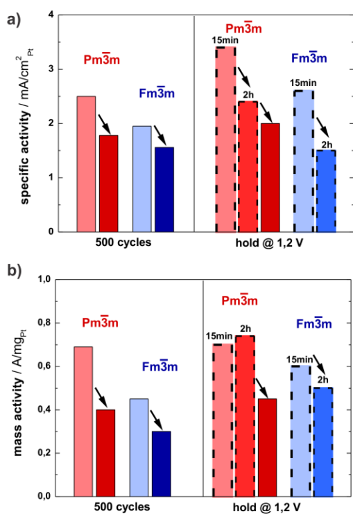
Figure 4. Comparison of a) specific and b) mass activities @ 0.9 V_{\text{RHE}} of the ordered (red) and the disordered (blue) catalysts after dealloying (500 cycles and potential hold @ 1.2 V for 15 min and 2 hours, respectively) and subsequent degradation (dark red and dark blue color). No subsequent degradation after holding the potential at 1.2 V_{\text{RHE}} was done for the disordered catalyst.
