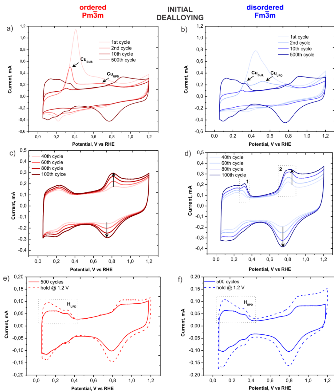
Figure 3. Selected cyclic voltammograms of the continuously recorded scans during dealloying with 500 cycles of the ordered Pm \bar{3} m (a, c; red) and the disordered Fm \bar{3} m (b, d; blue) catalyst, recorded at a scan rate of 0.2 Vs -1 . Comparison of the baseline scans of the ordered (e) and the disordered (f) catalyst after dealloying by cycling (solid line) and potential hold @ 1.2 V for 2 hours (dashed line), recorded at a scan rate 0.05 Vs -1 in 0.1 M HClO 4 .
