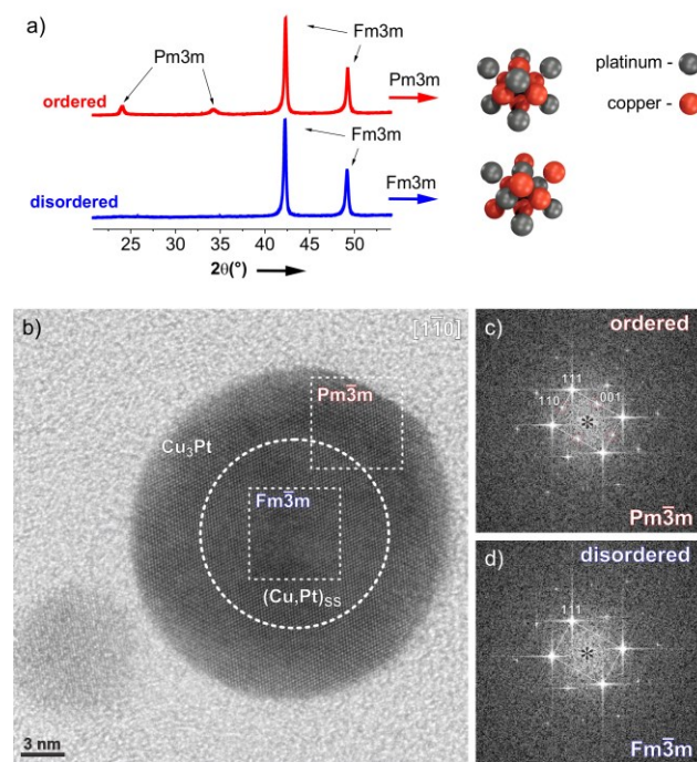
Figure 1. a) XRD patterns of ordered and disordered carbon supported PtCu 3 samples together with a representative Pm \bar{3} m and Fm \bar{3} m atomic arrangements, illustrated on the right. Structural analysis of partially ordered PtCu 3 nanoparticles. b) HRTEM image of a single PtCu 3 nanoparticle crystal oriented along the crystallographic [11-0] axis showing an apparent core-shell disordered-ordered structure. Averaged FFT power spectra for the (c) shell region with additional symmetry-specific Pm \bar{3} m reflections (indicated with 110 and 001); and the (d) core Fm \bar{3} m region without the super-structure reflections.
