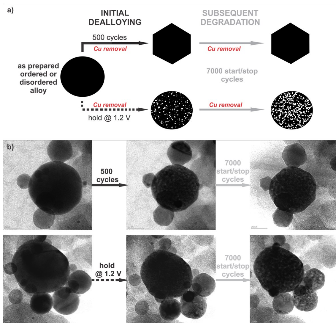
Figure 2: Electrochemical stability of the \text{PtCu}_3 nanocrystals. a) Schematic presentation of two types of electrochemical treatment protocols. Initial dealloying stage leads to a surface structure with reproducible activities, whereas the prolonged subsequent degradation gives a true insight into the stability of the catalyst. b) IL-TEM micrographs of disordered catalysts before, after initial dealloying and subsequent degradation. The upper sequence corresponds to dealloying with 500 potential cycles ( 1.2 \text{ V}_{\text{RHE}} upper limit), the lower one to dealloying with hold at 1.2 \text{ V}_{\text{RHE}} for 2 hours.
