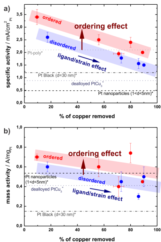
Figure 5: a) Specific activity and b) mass activity in relation to the copper content of the electrolyte upon different electrochemical treatments (dealloying and subsequent degradation). Activities of Pt-poly, Pt-black, dealloyed PtCu 3 and Pt nanoparticles are taken from references (*) 32 and (×) 18 .
