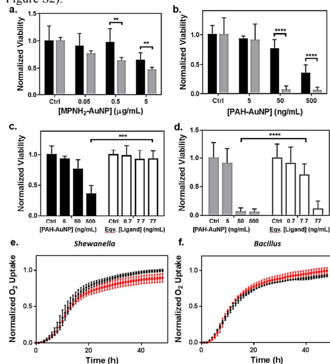
Figure 2. Bacterial viability assessed by colony counting methods (a-d) and respirometry (e-f). Dose-dependent toxicity assessment of (a) MPNH 2 -AuNPs and (b) PAH-AuNPs on Shewanella (black bars) and Bacillus (grey bars), and comparisons of toxicity between PAH-AuNPs and PAH free ligand on Shewanella (c) and Bacillus (d). Ligand concentrations were chosen based on XPS measurements of ligand coverage on nanoparticle surfaces. 31 Representative respirometry analysis of (e) Shewanella and (f) Bacillus without (black circles) and with (red squares) 5 \mu\text{g/mL} MPA-AuNPs in growth media. The O 2 consumption curve can be interpreted similarly to growth curves obtained through optical density measurements to assess the impact of NPs on the bacterial strains.
