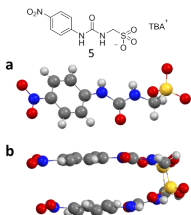
Figure 7 Single crystal X-ray structure of a) compound 5 which shows b) dimer formation through urea-anion hydrogen bond formation. The TBA counter cation and second sulfonate urea anion have been omitted for clarity where necessary. Nitrogen atoms blue, hydrogen atoms white, carbon atoms grey, oxygen atoms red, sulphur atoms yellow and fluoride atoms green. Crystals were obtained by slow evaporation of a chloroform solution containing 5 .
