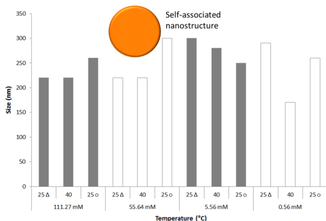
Figure 5 Maxima observed from DLS average intensity size distributions (as shown in Figure 4) for 1 at varying concentrations and temperatures. 25 Δ - readings taken at 25 °C before heating to 40 °C; 25 ○ - readings taken at 25 °C after heating to 40 °C.
