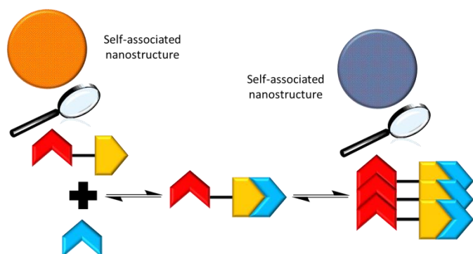
Scheme 3 Summary of the proposed hydrogen bonded complexes formed from solutions of 1 and solutions of 1 and 2 in DMSO, based on the NMR evidence presented herein.
