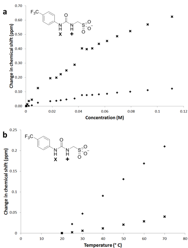
Figure 2 a) Graph illustrating the ^1\text{H} NMR down-field change in chemical shift of urea NH resonances with changing concentration of 1 in \text{DMSO-}d_6/0.5\% \text{H}_2\text{O} (298 K); b)
