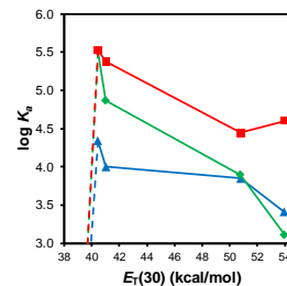
Fig 2. Binding constant of 2 (■), 3 (◆), and 4 (▲) by host 1a as a function solvent polarity. The actual binding constants are reported in Table S2. The data points are connected to guide the eye. Binding in 3:2 hexane/DCM was too weak to be measured accurately.
