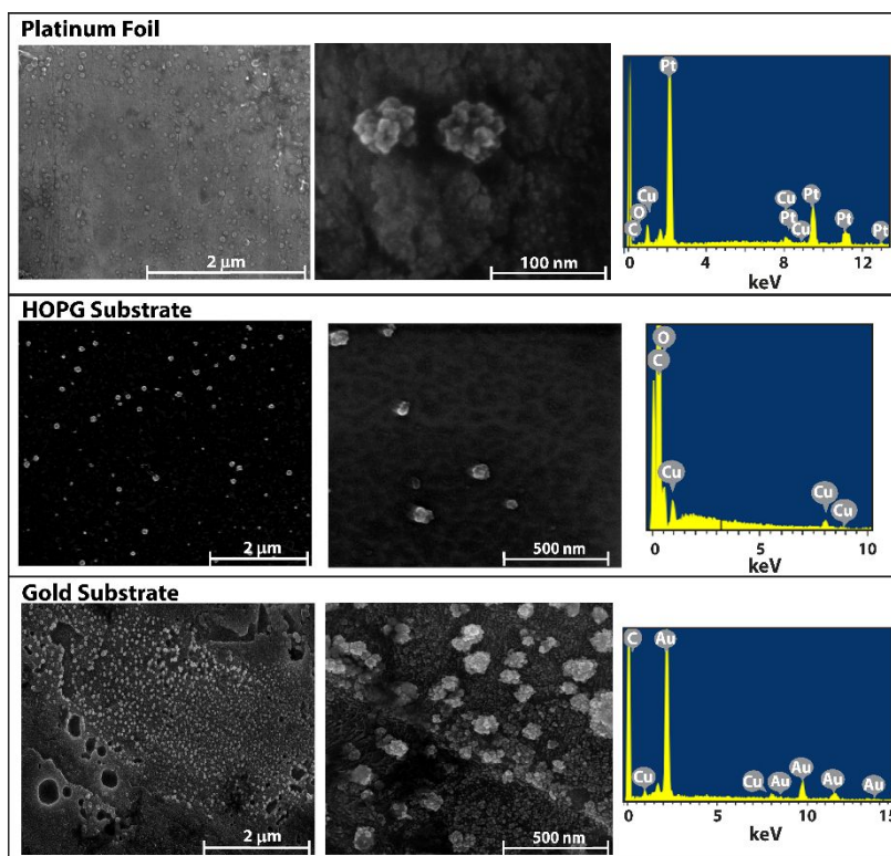
Figure 1. SEM images and representative EDX spectra showing the morphologies of copper nanoparticles (NPs) deposited on a variety of substrates such as: platinum foil, highly oriented pyrolytic graphite (HOPG), and gold. Nanoparticles were deposited from aqueous nanodroplets containing 50 mM \text{CuCl}_2 in a continuous phase of 0.1 M [\text{TBA}][\text{PF}_6] in 1,2-DCE.
