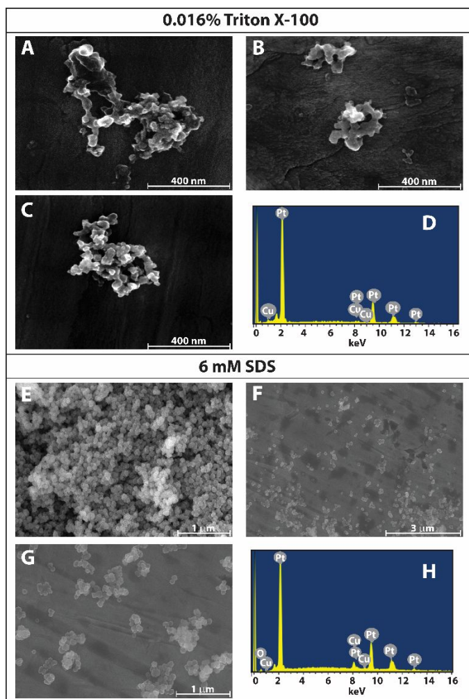
Figure 3. SEM images and representative EDX spectra showing the morphologies of copper nanoparticles (NPs) deposited on platinum foil from aqueous nanodroplets containing 50 mM \text{CuCl}_2 with added surfactants in a continuous phase of 0.1 M [\text{TBA}][\text{PF}_6] in 1,2-DCE. (A-D) SEM data and corresponding EDX using an added surfactant of 0.016% w/v Triton X-100. (E-H) SEM data using an added surfactant of 6 mM SDS ( r = 28 \text{ nm} \pm 11 \text{ nm} ).
