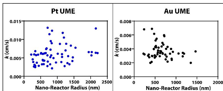
Figure 2. Plots demonstrating the effect that aqueous nanodroplet size, filled with 50 mM \text{CuCl}_2 and glycerol (50%, v/v), has on the heterogeneous rate kinetics on a Pt and Au microelectrode. The large spread in the data without an
