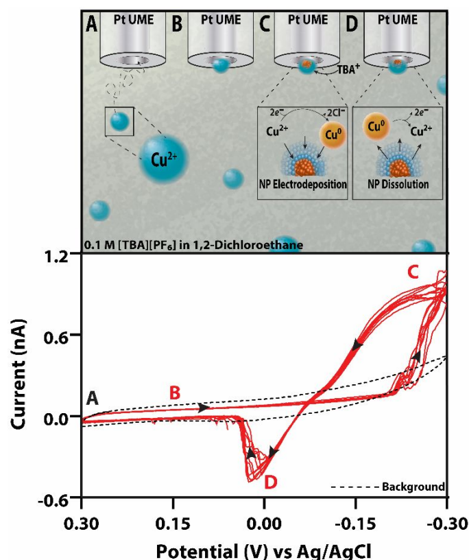
Figure 4. Representative cyclic voltammogram of the electrodeposition and anodic stripping of a copper nanoparticle deposited from aqueous nanodroplets filled with 50 mM \text{CuCl}_2 suspended in a 0.1 M \text{TBAPF}_6 in DCE continuous phase on a Pt microelectrode ( r \sim 5 \mu\text{m} ). Showing (A) the aqueous \text{Cu}^{2+} containing reactor diffusing in solution (B) the reactor initially colliding with the Pt UME (C) the \text{Cu}^{2+} being reduced to a \text{Cu}^0 nanoparticle at sufficiently negative potentials before (D) undergoing anodic stripping.
