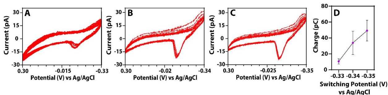
Figure 5. Cyclic voltammograms and overall trend of a single 50 mM \text{CuCl}_2 nanodroplet in a solution of water saturated 1,2-DCE on a Pt UME ( r \sim 5 \mu\text{m} ) versus Ag/AgCl at a scan rate of 0.025 V/s showing a distinct increase in charge as the switching potential is made more negative from (A) -0.33 V to (B) -0.34 V to (C) -0.35 V. (D) Overall trend of the integrated charge of the oxidative stripping peak as a function of switching potential with each point including data from >20 stripping peaks.
