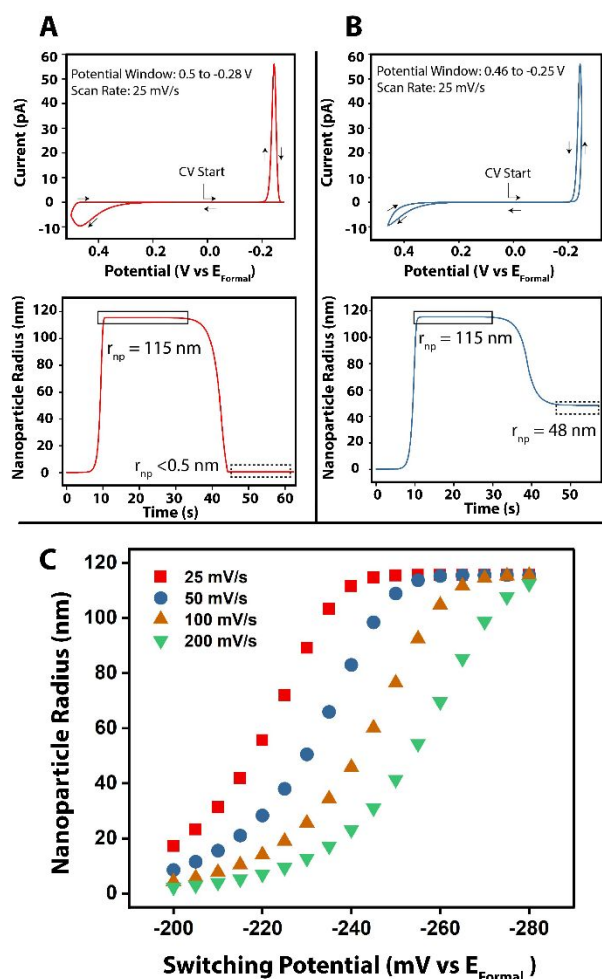
Figure 6. A) Simulated cyclic voltammogram of a 1.3 \mu\text{m} aqueous nanodroplet with 50 \text{ mM Cu}^{2+} precursor ion demonstrating hemispherical nanoparticle electrodeposition and oxidative stripping. The nanoparticle growth curve is presented below, demonstrating an initially rapid complete nanoparticle growth under sufficient cathodic potentials and gradual complete nanoparticle dissolution under sufficiently anodic conditions. B) Representative simulated cyclic voltammogram with hemispherical nanoparticle electrodeposition ( vide supra ) under different voltammetric conditions, revealing significant changes in the i - E profile and nanoparticle growth profile including a rapid complete growth and a gradual incomplete dissolution. C) Simulated hemispherical Cu nanoparticle radii at a range of voltammetric switching potentials and scan rates during the cathodic electrodeposition sweep, allowing both complete and incomplete precursor electrolysis in the reactor.
