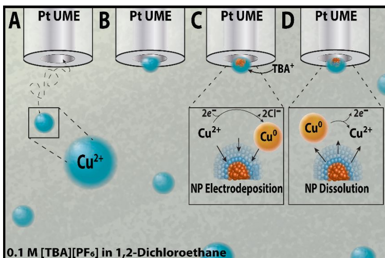
Scheme 1. Representation of the electrodeposition and anodic stripping of a copper nanoparticle deposited using aqueous nanodroplets filled with 50 mM CuCl 2 on a Pt microelectrode (UME, r \sim 5 \mu\text{m} ). Showing (A) the aqueous Cu 2+ containing reactor diffusing in solution (B) the reactor initially colliding with the Pt UME (C) the Cu 2+ being reduced to a Cu 0 nanoparticle and its corresponding reaction before (D) experiencing nanoparticle dissolution.
