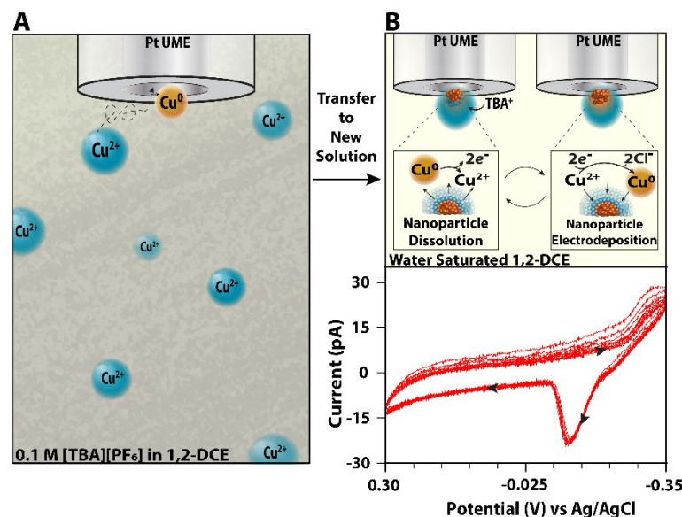
Scheme 2. Representation of the single nanodroplet isolation experiment. (A) A 50 mM \text{CuCl}_2 aqueous nanodroplet suspended in 1,2-DCE with 0.1 M [\text{TBA}][\text{PF}_6] first diffusing to the Pt UME ( r \sim 5 \mu\text{m} ) before being electrodeposited at a scan rate of 0.2 V/s. The cyclic voltammogram is then stopped and the Pt UME with the single droplet is placed in a solution of water saturated 1,2-DCE. (B) Schematic and voltammogram of the single reactor repeatedly going through oxidative stripping and electrodeposition at a scan rate of 0.025 V/s and switching potential of -0.35 V.
