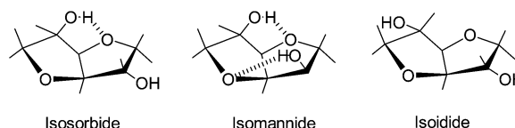
Fig. 1 The three diastereoisomers of dianhydrohexitols.
