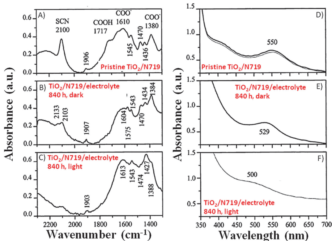
Fig. 4 FTIR (left side) and UV-Vis (right side) spectra of: (A, D) non-treated working electrodes in an Ar atmosphere; (B, E) working electrodes being soaked in a liquid electrolyte (LiI 0.50 M and \text{I}_2 50 mM in MPN) with 5 vol% \text{H}_2\text{O} under dark for 840 h; (C, F) working electrodes being soaked in the same liquid electrolyte under visible light illumination for 840 h. FTIR spectra of the treated samples were normalized based on the \text{TiO}_2 absorption maximum of the reference sample at 832\text{ cm}^{-1} . Adapted and reprinted from ref. 85.
