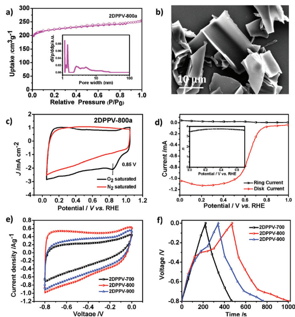
Fig. 3 (a) Nitrogen adsorption–desorption isotherms of 2DPPV-800a (inset: pore size distribution); (b) SEM image of 2DPPV-700; (c) CV curves of 2DPPV-800a in N_2 -saturated and O_2 -saturated 0.1 M KOH at a scan rate of 50\text{ mV s}^{-1} ; (d) RRDE voltammogram for 2DPPV-800a in 0.1 M KOH solution saturated with O_2 (the electrode rotation rate was 1600 rpm and the Pt ring electrode was held at 0.5 V, inset: electron transfer number of 2DPPV-800a as a function of potential); (e) CV curves of 2DPPV- X ( X = 700, 800, 900 ) at 5\text{ mV s}^{-1} in 6 M KOH aqueous solution; and (f) galvanostatic charge/discharge curves for 2DPPV- X ( X = 700, 800, 900 ) at a current density of 0.5\text{ Ag}^{-1} .
