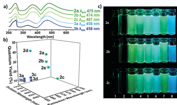
Fig. 1 (a) UV and emission spectra of fluorescent aminomaleimides (2a–c) and alkoxybromomaleimides (3a–b); (b) fluorescence quantum yields of the singly substituted maleimides (2a–e, 3a–d) against excitation and emission wavelengths (recorded at 10 \mu M in diethyl ether); (c) aminomaleimides (2a–c) in 8 solvents (1–8: H 2 O, MeOH, DMF, dioxane, THF, Et 2 O, CH 2 Cl 2 and cyclohexane) under UV light (365 nm).
