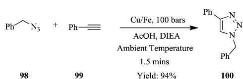
Scheme 23 Cu–Fe catalysed synthesis of triazoles via azide–alkyne cycloaddition.
