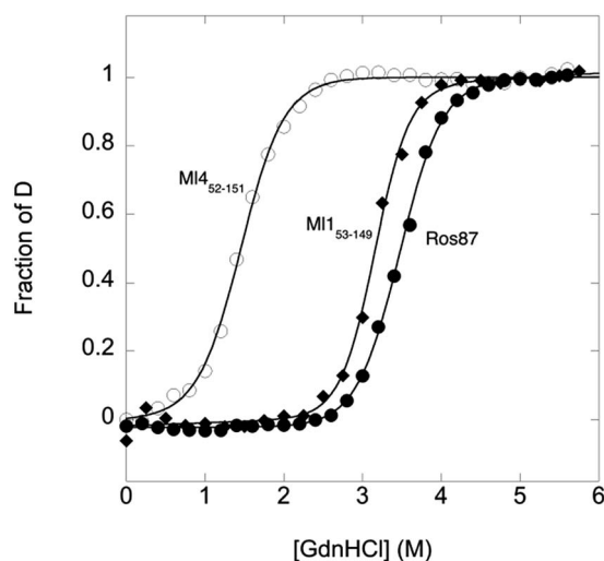
Fig. 2 GdnHCl-induced equilibrium denaturation of Ros87, Ml1 53-149 and Ml4 52-151 at 298 K and pH 6.8 using 20 mM sodium phosphate, 300 mM NaCl, 100 \mu M ZnCl 2 , and 4 mM TCEP, as a function of intrinsic tryptophan emission.
