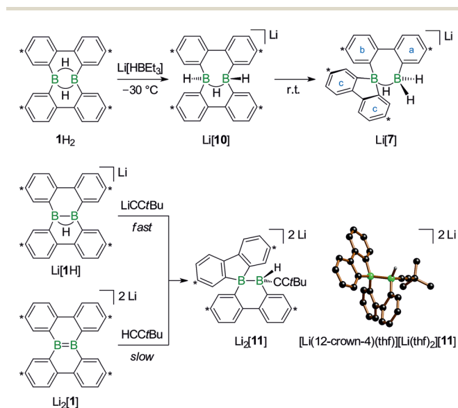
Scheme 6 Reaction of 1H 2 with Li[HBET 3 ] at −30 °C to give Li[10], which isomerizes to Li[7] at room temperature (top). Compound Li 2 [11] forms in both reactions, t BuCCl/Li[1H] and t BuCCl/Li 2 [1] (bottom; carbon atoms marked with asterisks bear t Bu substituents). Molecular structure of [Li(12-crown-4)(thf)][Li(thf) 2 ][11] in the solid state. The solvent-separated cations, phenyl-bonded t Bu groups, and all CH atoms are omitted for clarity.
