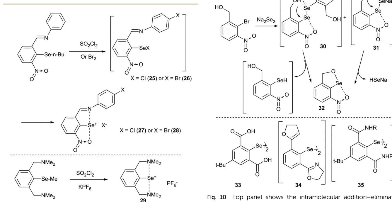
Fig. 9 Ionization of selenenyl halides.
