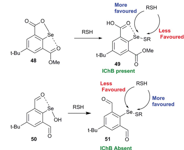
Fig. 22 Steric confinement with adaptive rotor characteristics prevents IChB and favours the nucleophilic attack on sulfur.
