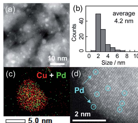
Fig. 1 (a) HAADF-STEM image of Cu 5 Pd/Al 2 O 3 and (b) size distribution of the nanoparticles. (c) Elemental map of the Pd + Cu overlay, as acquired by EDS. (d) High-resolution image of a single nanoparticle.
