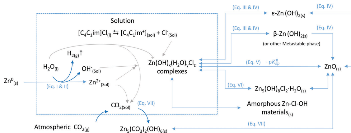
Fig. 9 General conversion paths of metallic zinc into ZnO in [\text{C}_4\text{C}_1\text{im}]\text{Cl} /water systems. Equations in the scheme are not balanced. Equations are given in the text. The predominant path and species formed will depend on the temperature and water content.
