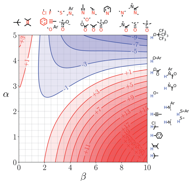
Fig. 6 FGIP for the interaction of two solutes in 1,1,1,3,3,3-hexafluoro-2-propanol at 298 K ( \Delta\Delta G_{\text{FGI}} in kJ mol -1 ). The solute-solute interactions in the blue region, and unfavourable in the red region.
