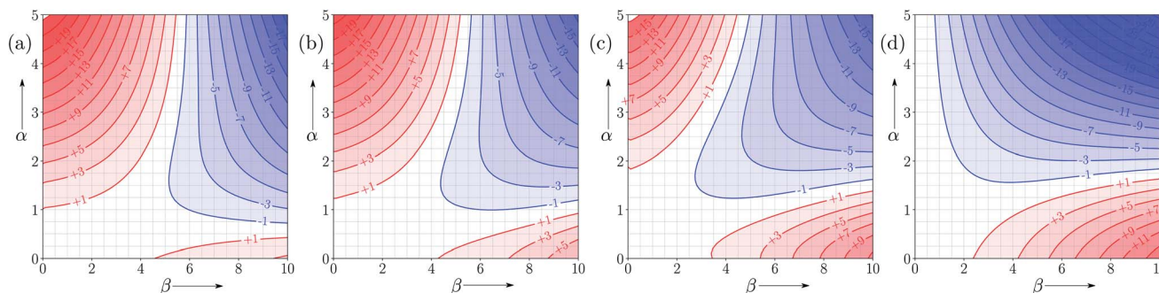
Fig. 10 FGIs for the interaction of two solutes in (a) 100% THF 0% chloroform (b) 70% THF 30% chloroform (c) 30% THF 70% chloroform (d) 0% THF 100% chloroform mixtures by volume at 298 K ( \Delta\Delta G_{\text{FGI}} in \text{kJ mol}^{-1} ). The solute–solute interactions are favourable in the blue region, and unfavourable in the red region.
