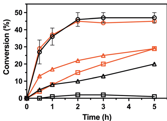
Fig. 4 Conversion in the kinetic resolutions of ( R,S )-PEA (circle) and ( R,S )-PPA (triangle), as well as the deamination of ( R )-PBA (square), using pyruvate as the amine acceptor from the LS_ATA wild-type (black) and the V37A variant (red). All experiments were performed at least in duplicate. Errors smaller than symbols are not presented. Experimental details are found in the ESI.†
