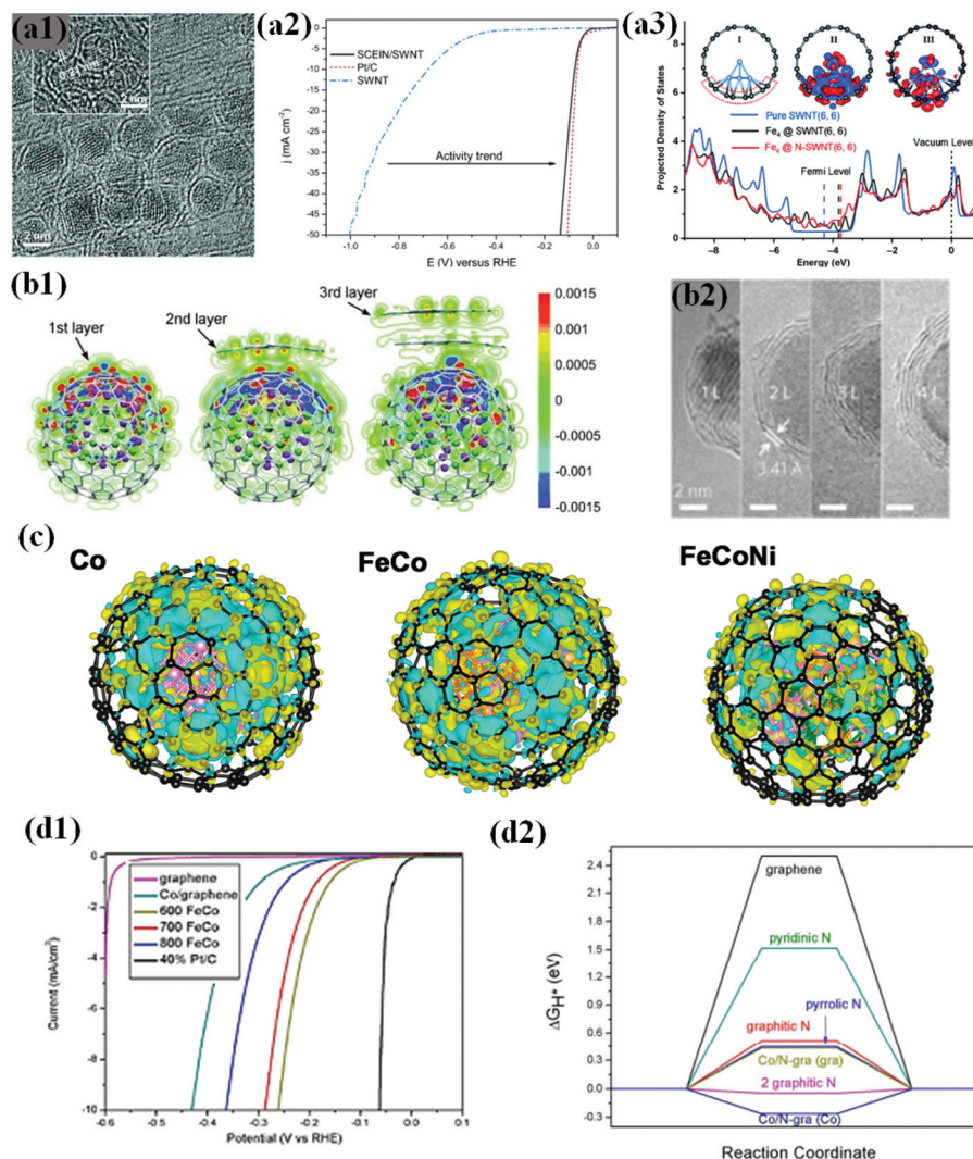
Fig. 4 (a1) HRTEM image of the SCEIN/SWNT sample, the inset indicates the (110) lattice plane of the Fe particles in Science. (a2) Polarization curves of SWNT (blue), SCEIN/SWNT (black), and Pt/C (red). The polarization curves were measured at a scan rate of 50 \text{ mV s}^{-1} in 0.5 \text{ M H}_2\text{SO}_4 , reproduced with permission from ref. 66, Wiley publications, copyright 2015. (a3) Projected DOS of the p orbitals of C atoms bonded to \text{Fe}_4 in \text{Fe}_4 @SWNT and \text{Fe}_4 @N-SWNT compared with that in pure SWNT. Inserted plot I and plot II show the optimized structure of \text{Fe}_4 @SWNT and its difference charge density, and plot III corresponds to that of \text{Fe}_4 @N-SWNT. The red and blue regions in plots II and III indicate a charge increase and decrease, respectively, reproduced with permission from ref. 109, Wiley publications, copyright 2018. (b1) HRTEM images of \text{CoNi@NC} , showing the graphene shells and encapsulated metal NPs. Inset: Crystal (111) plane of the \text{CoNi} alloy. (b2) Redistribution of the electron densities after the \text{CoNi} clusters are covered by one to three layers of graphene. The red and blue regions are regions of increased and decreased electron density, respectively, reproduced with permission from ref. 113, Wiley publications, copyright 2015. (b3) High-resolution transmission electron microscopy (HRTEM) images of \text{FeCo} NPs covered by one to four layers of graphene (1–4 L), reproduced with permission from ref. 114, RSC publications, copyright 2013. (c) Calculated charge density differences of various models. The isosurface value of the color region is 0.01 \text{ e } \text{\AA}^{-3} . The yellow and cyan regions refer to increased and decreased charge distributions, respectively. \text{FeCoNi} ( \text{Fe}_{24}\text{Co}_{24}\text{Ni}_7 ) refers to ternary alloys with lower and higher Ni contents, respectively, reproduced with permission from ref. 119, ACS publications, copyright 2017. (d1) Polarization curves of different \text{FeCo} annealed samples measured at a scan rate of 50 \text{ mV s}^{-1} in 0.5 \text{ M H}_2\text{SO}_4 solution. (d2) Calculated \Delta G_{\text{H}^+} diagram of some models; the words in the bracket mean the \text{H}^* adsorbed on whether graphene or \text{Co}_4 side, reproduced with permission from ref. 76, RSC publications, copyright 2015.
