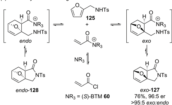
Scheme 28 Organocatalytic Diels-Alder-lactamization.
