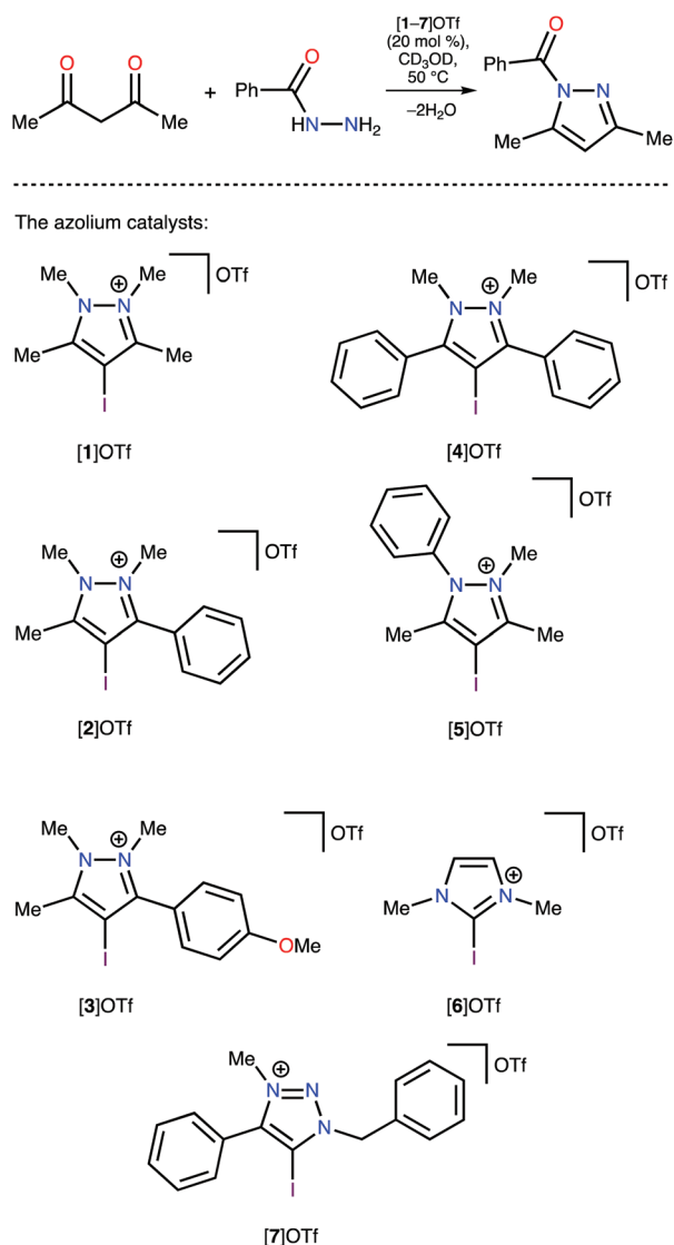
Scheme 2 The series of azolium catalysts tested in the Knorr-type reaction.
