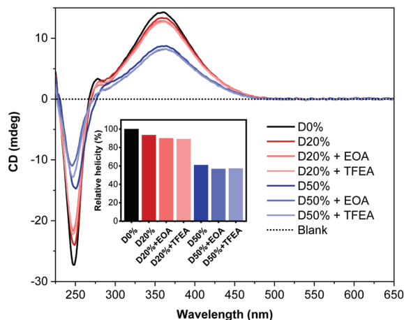
Fig. 7 CD (THF, 0.5 mg mL^{-1} ) spectra of D0% , D20% , and, D50% before and after treatment with EAO or TFEA and purification by dialysis. The inset shows the helicity (CD at \lambda = 360 nm) of the copolymers compared to D0% .
